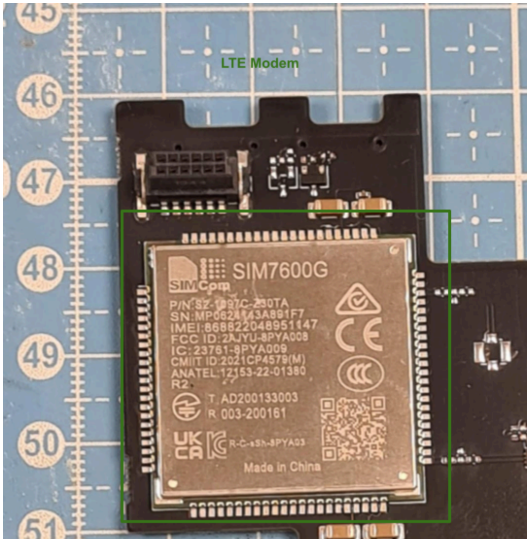
Photo 8 - LTE MODEM - Detail
