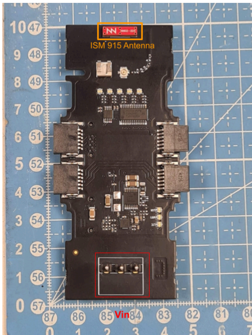
Photo 1 - Front Board - Top
