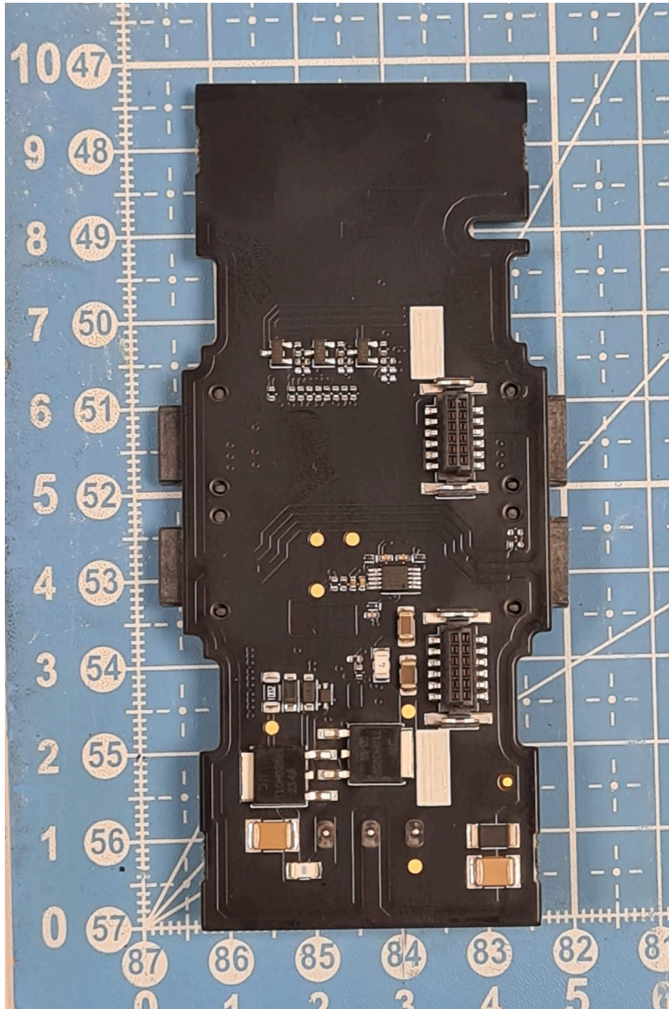
Photo 2 - Front Board - Bottom
