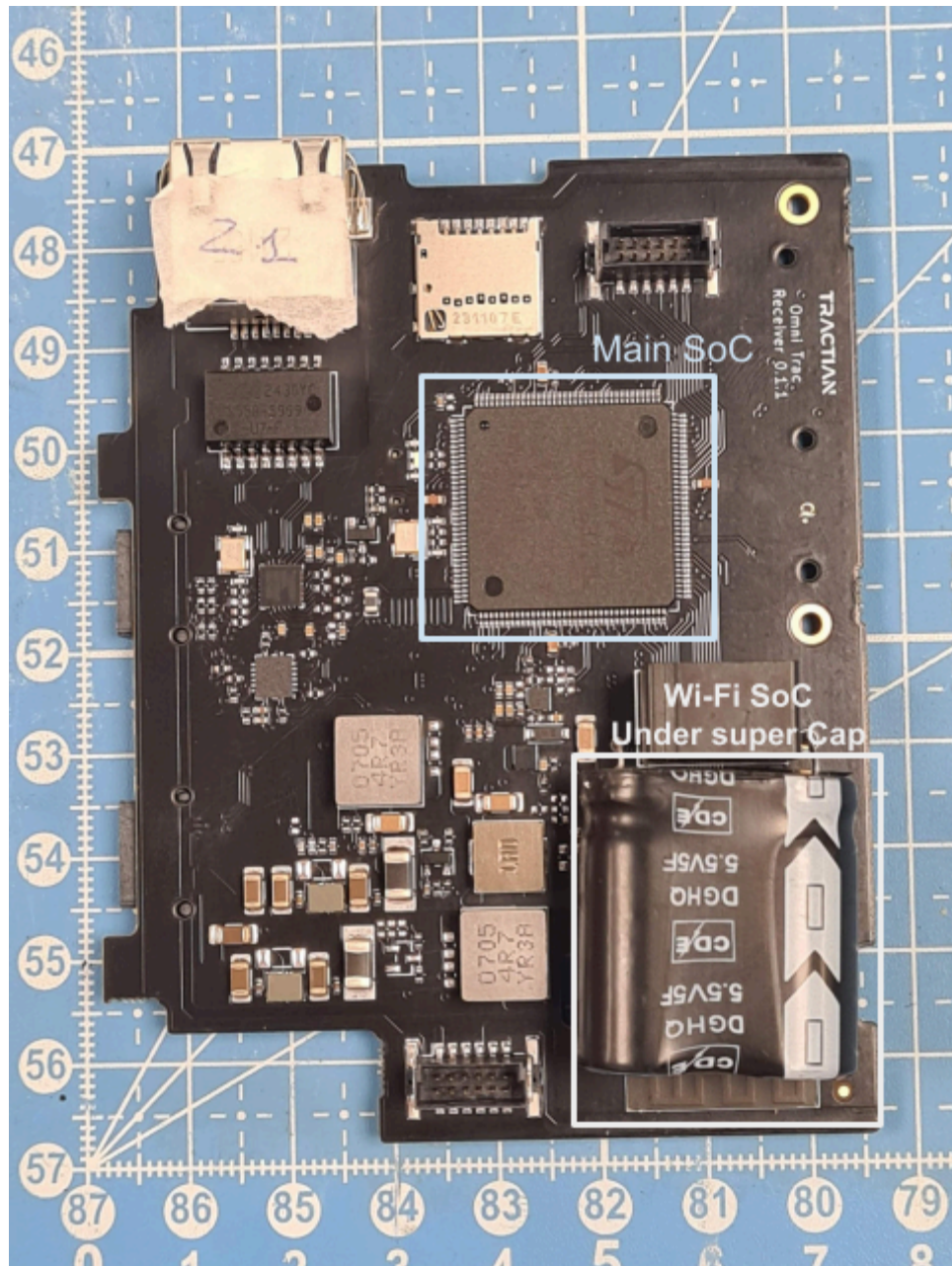
Photo 4 - Main Board - top
