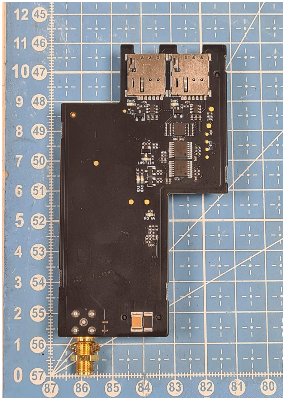
Photo 9 - Cellular Board - Bottom
