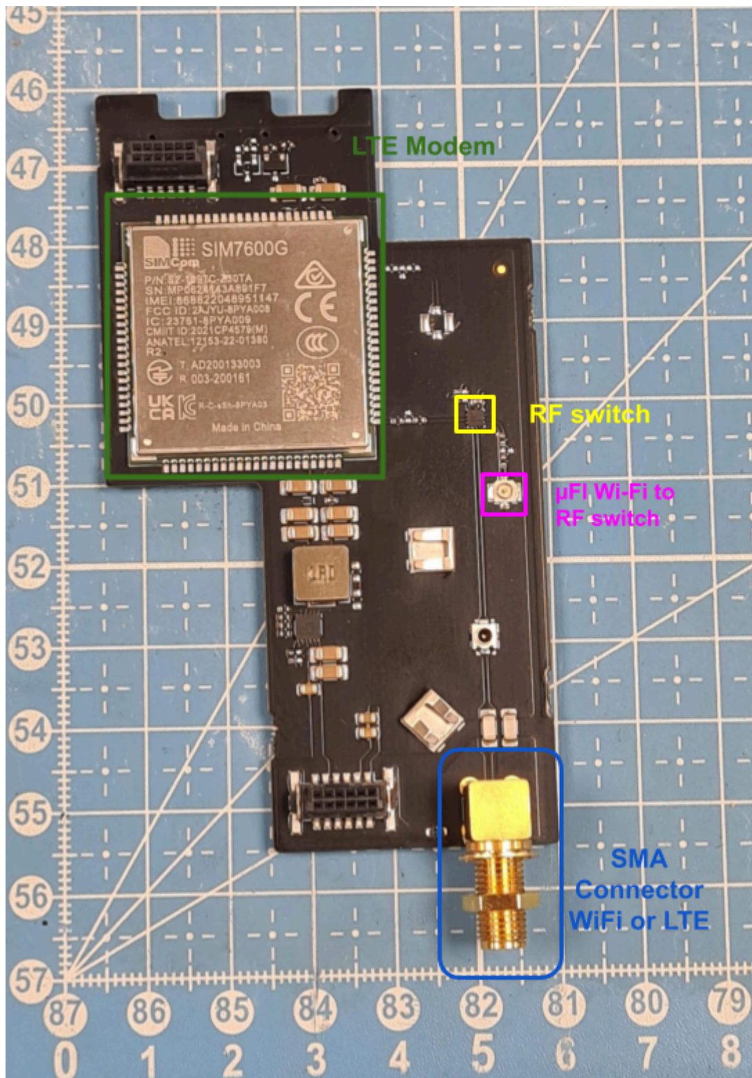
Photo 7 - Cellular Board - Top
