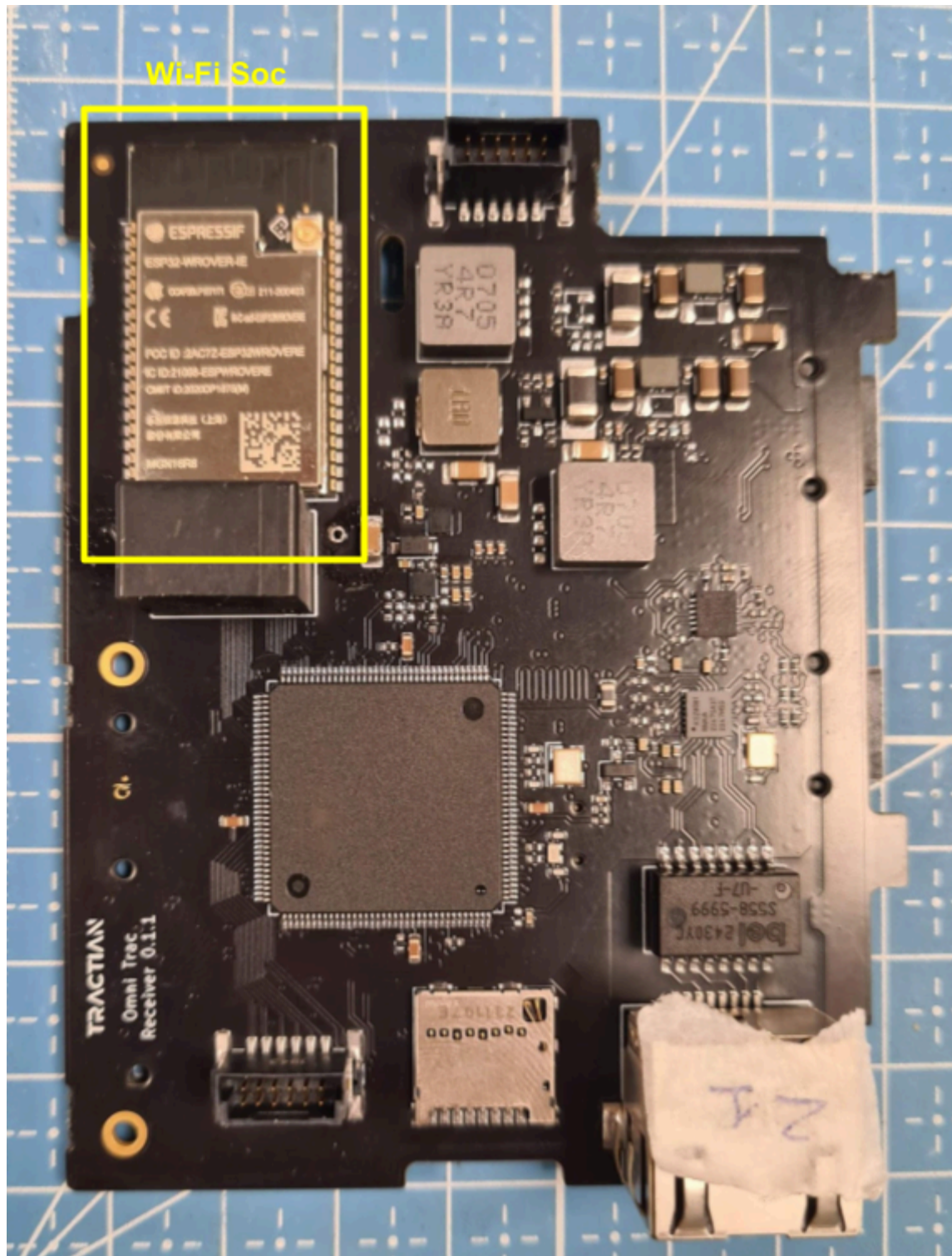
Photo 5 - Main Board without SuperCap - top
