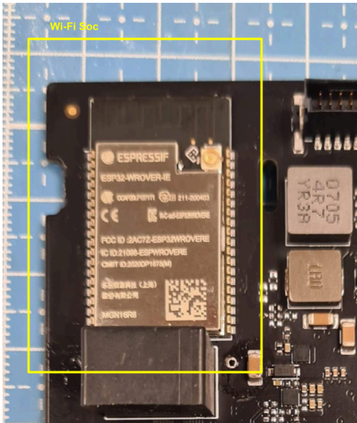
Photo 6 - Wi-Fi SoC - Detail
