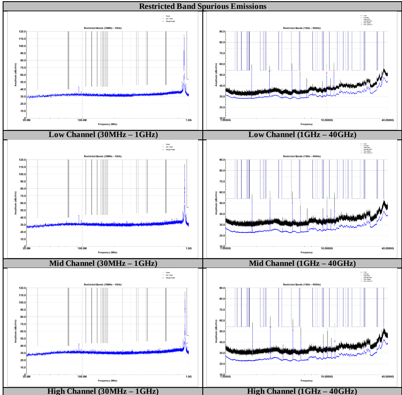
Figure 18. 30MHz – 40GHz Restricted Band Spurious Emissions
