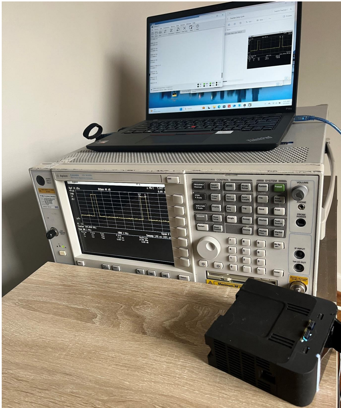
Conducted Tests at the Antenna Port
