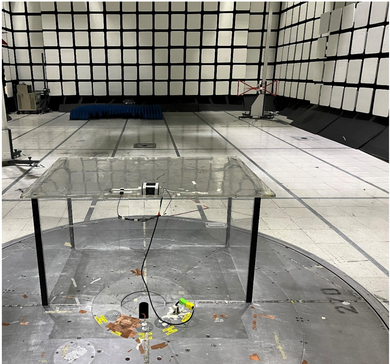
Radiated Emissions, 30MHz – 1GHz (Back Side)
