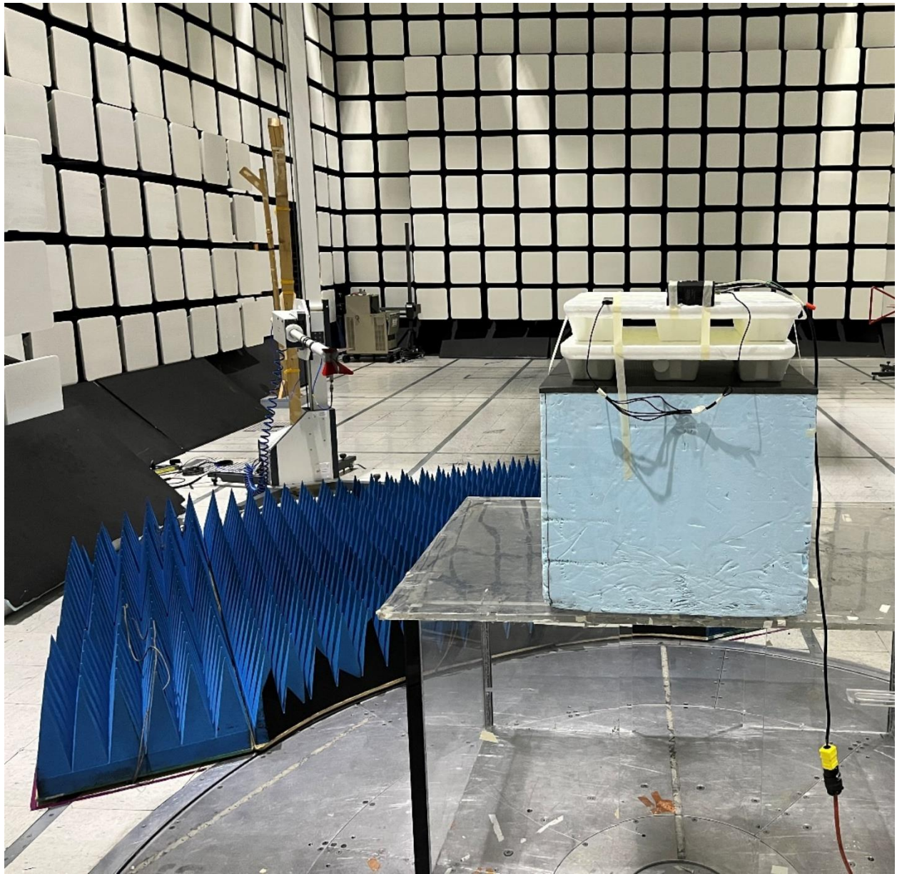
Radiated Emissions, Above 1GHz (Back Side)
