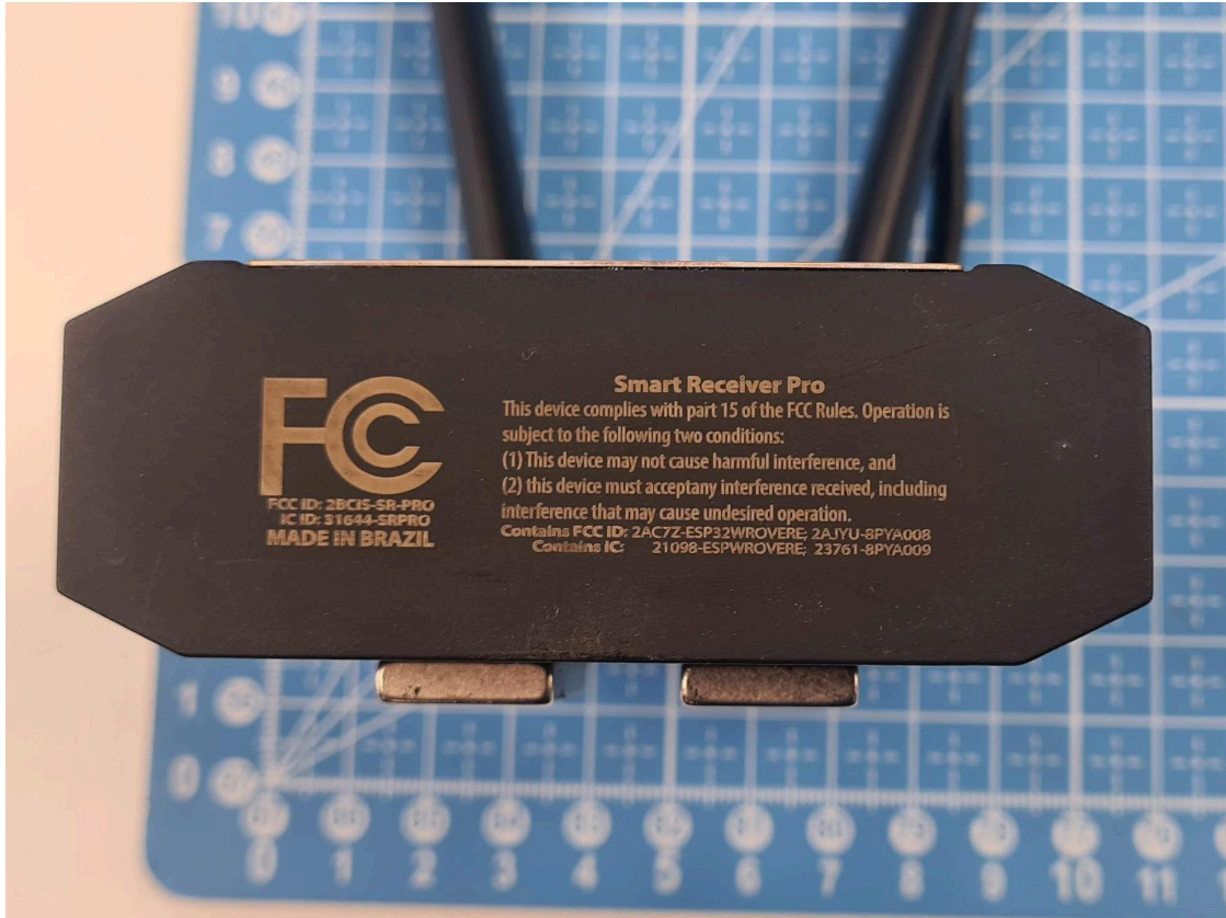
Figure 4 - Smart Receiver Pro - Bottom
