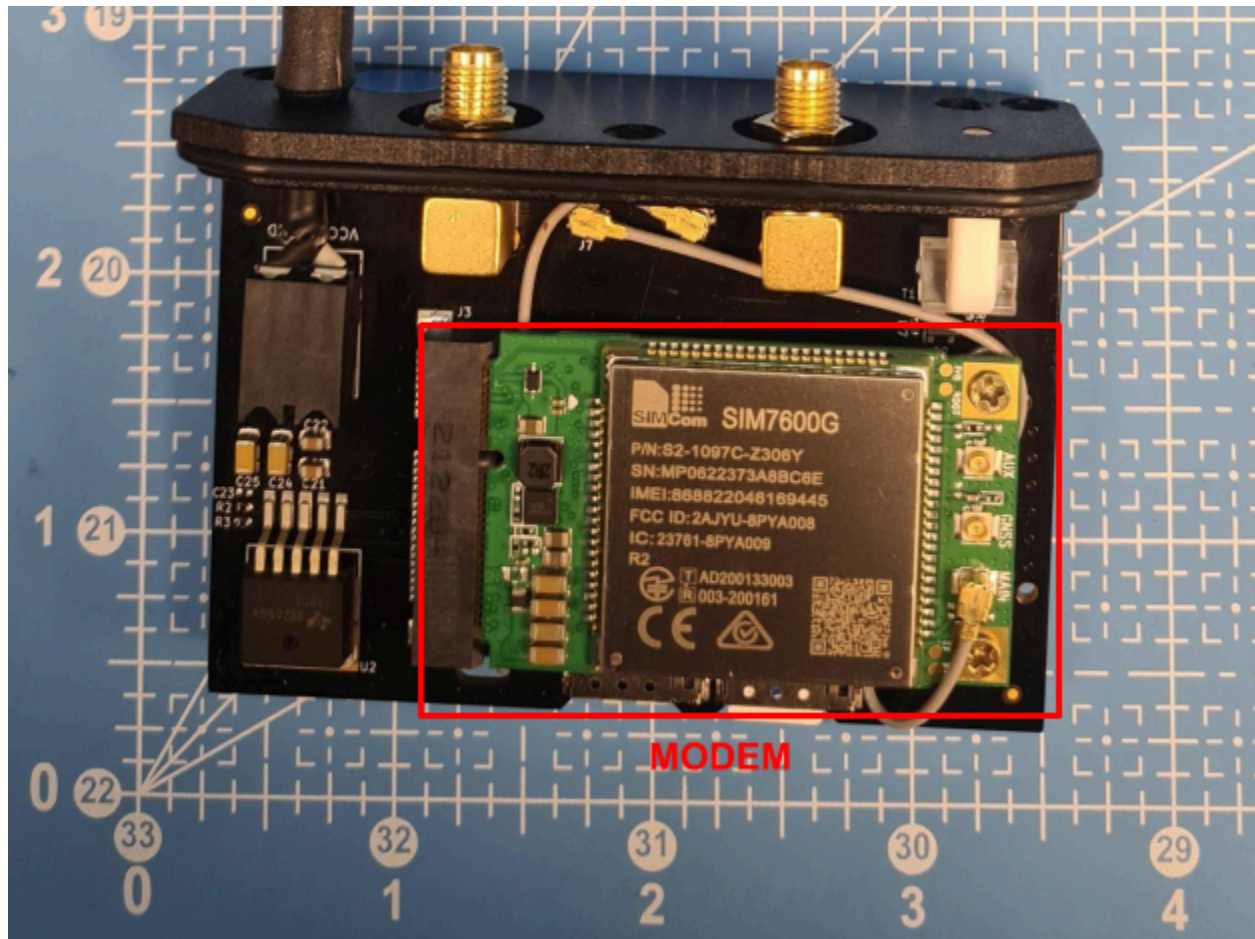
Figure 1 - Top View - Internal
