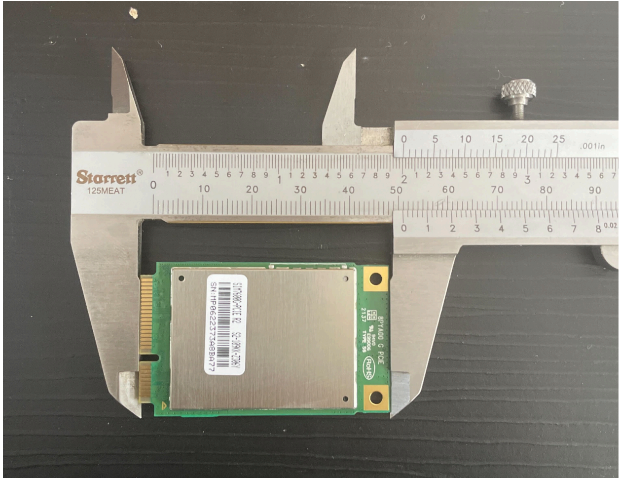
Figure 4 - Modem SIM7600G - Bottom
