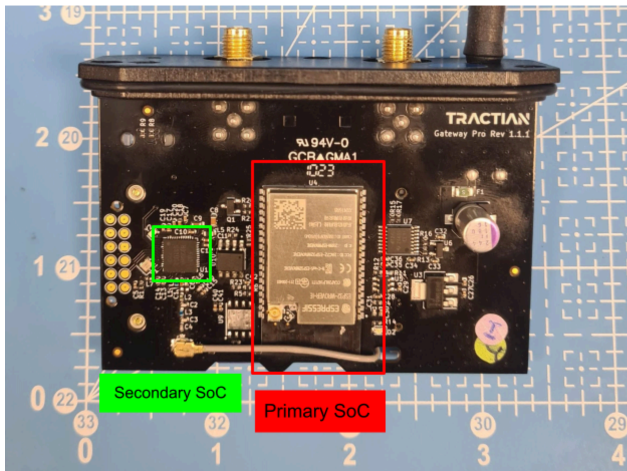
Figure 2 - Bottom View - Internal
