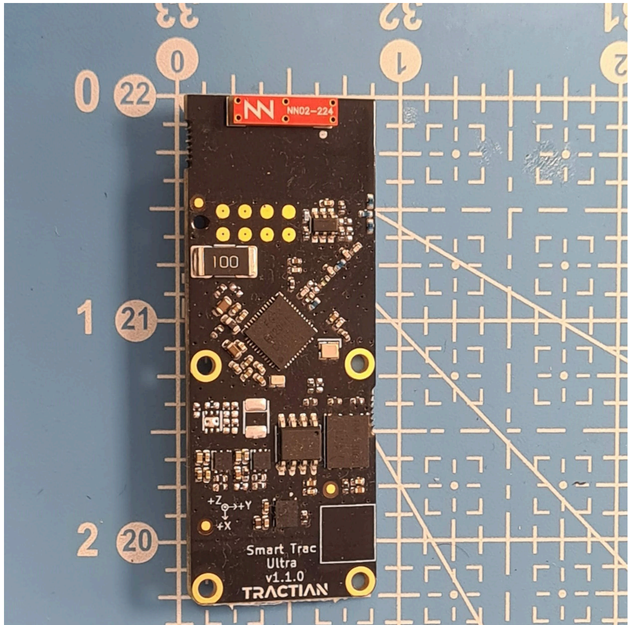
Figure 5 - Smart Trac Ultra - PCB - Top View
