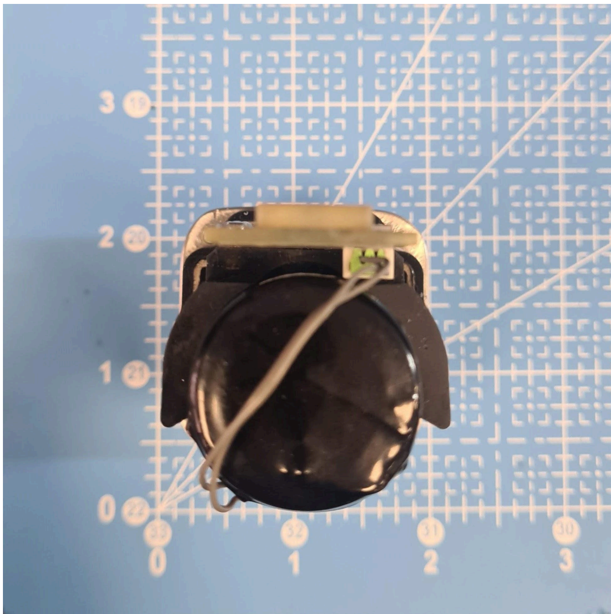
Figure 2 - Smart Trac Ultra - Internal - Top View
