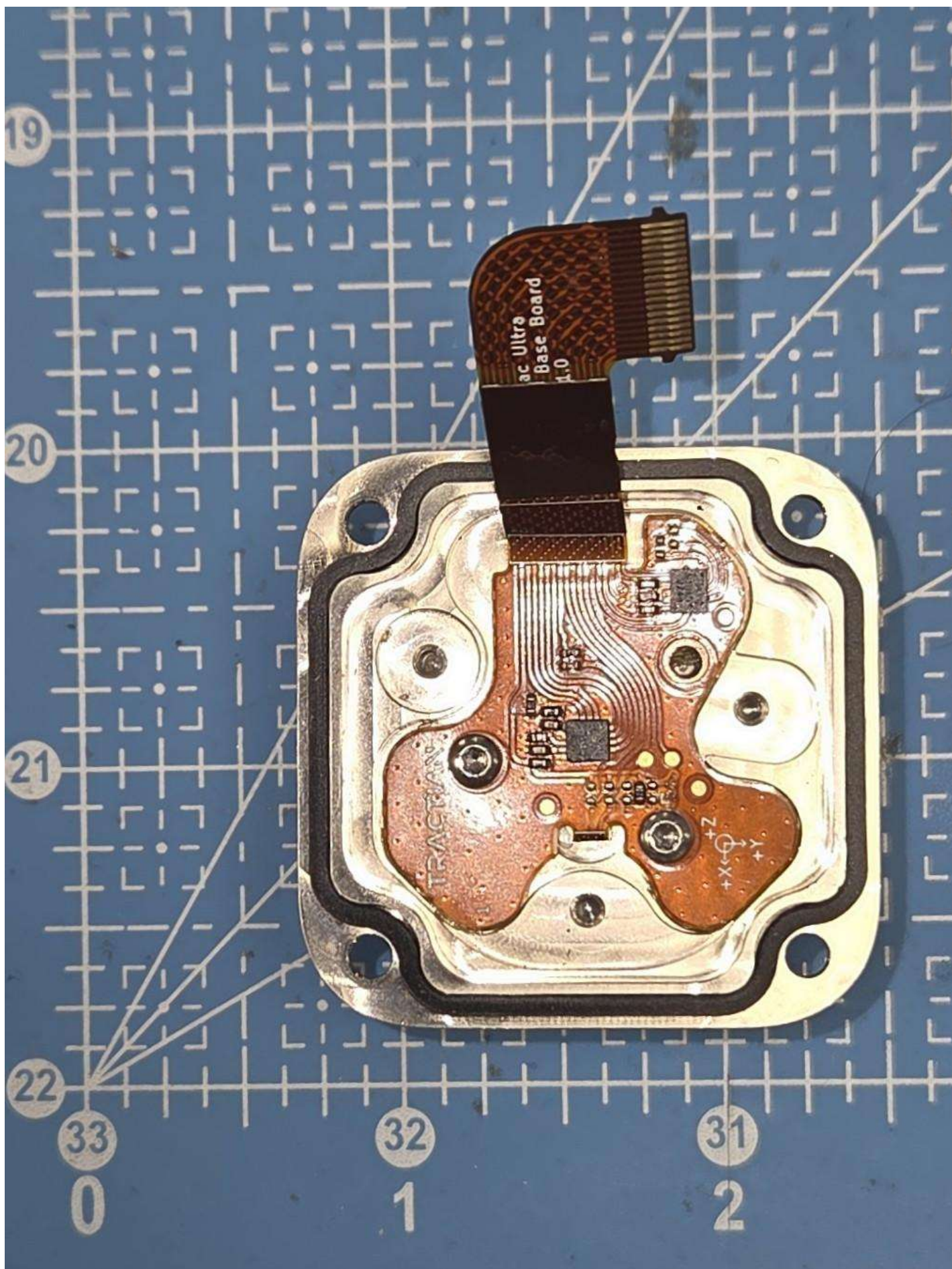
Photo 06 - Internal Photo - PCB assembled on the base
