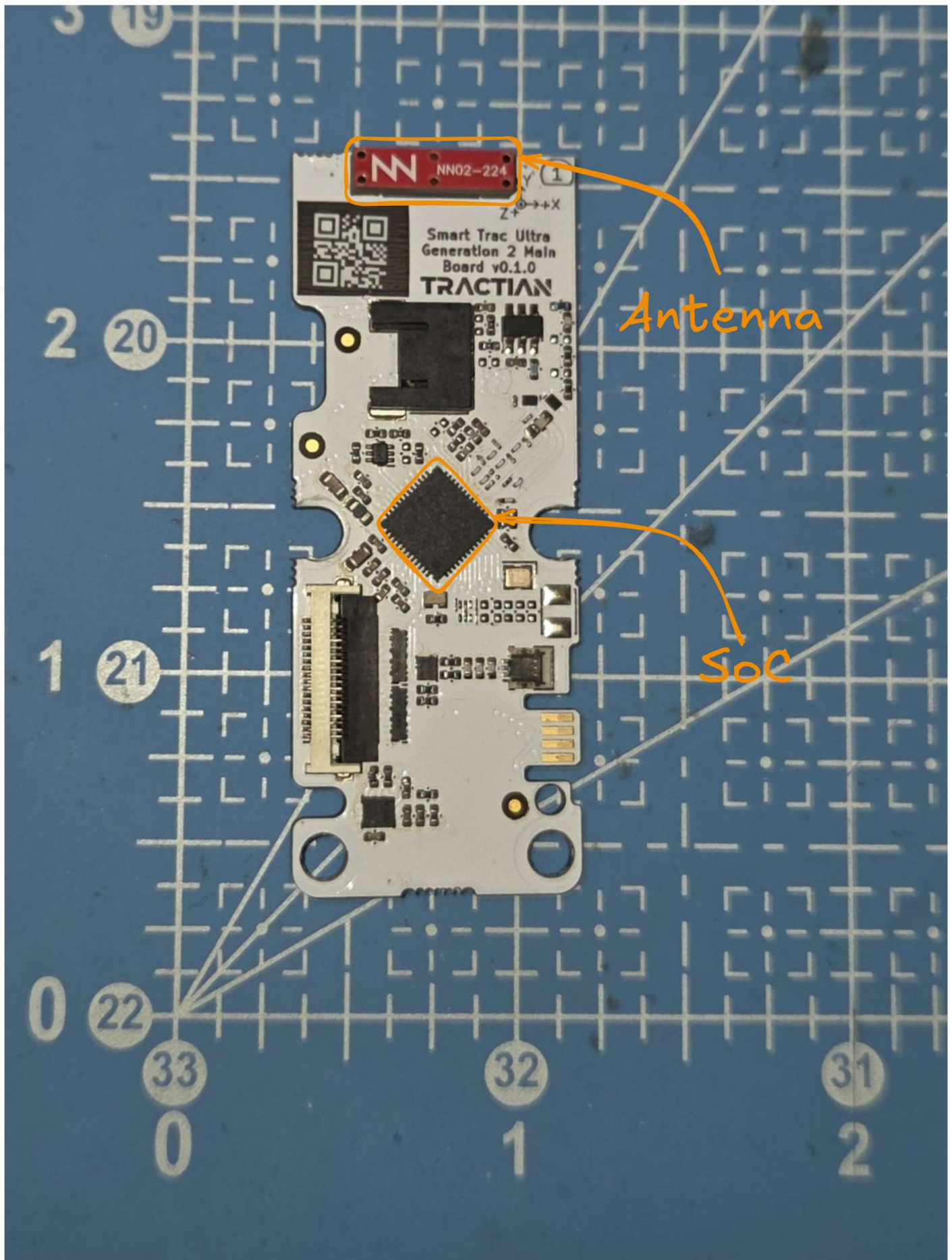
Photo 07 - Internal Photo - Main PCB - Top
