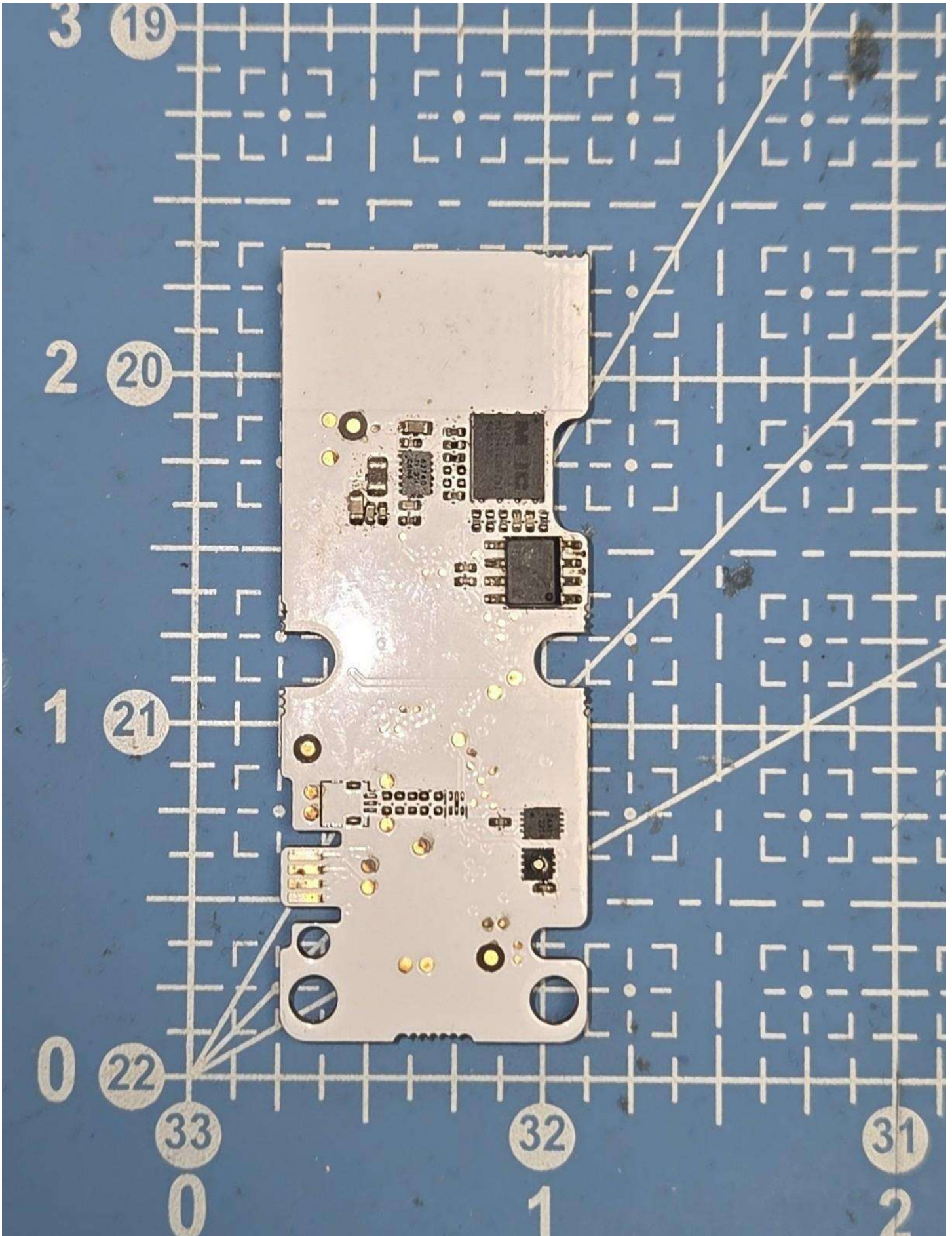
Photo 08 - Internal Photo - Main PCB - Bottom
