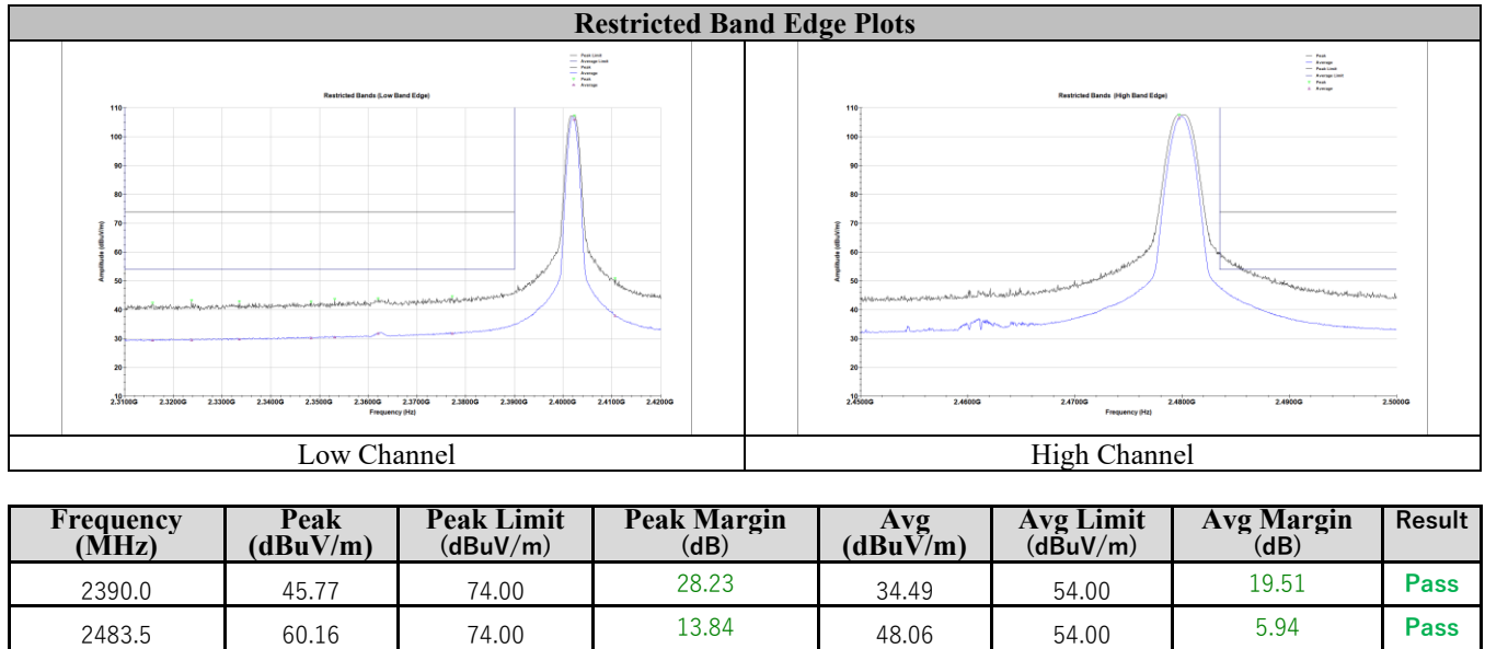
Figure 9. Restricted Band Edge Spurious Emissions (Low and High Band Edge)
