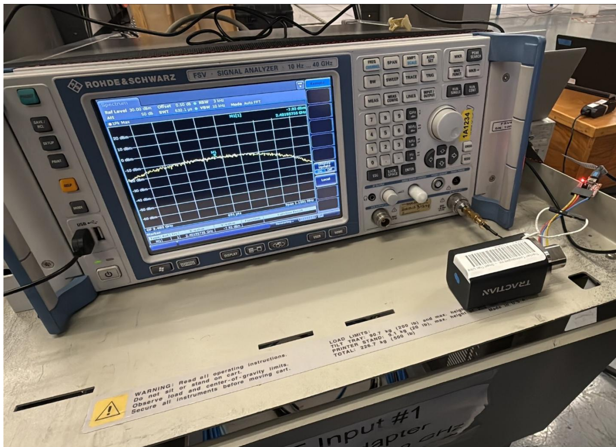
Conducted Antenna Port Measurements
