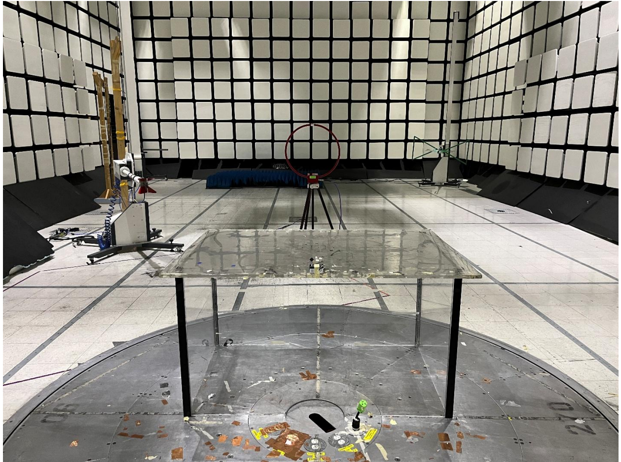
Radiated Emissions Below 30MHz (Back Side)
