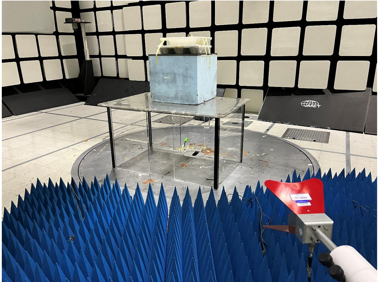
Radiated Emissions Above 1GHz (Antenna View)
