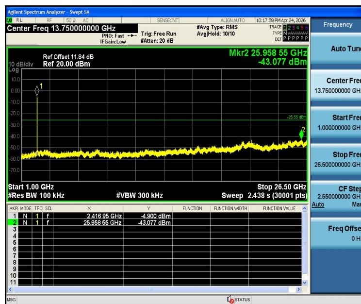
11AX40SISO-Ant2-2437-0~Reference-PASS
