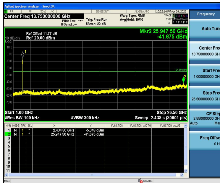
11AX40SISO-Ant2-2452-0~Reference-PASS
