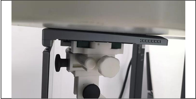
Laptop mode Bottom Side (Separation distance of 0mm)
