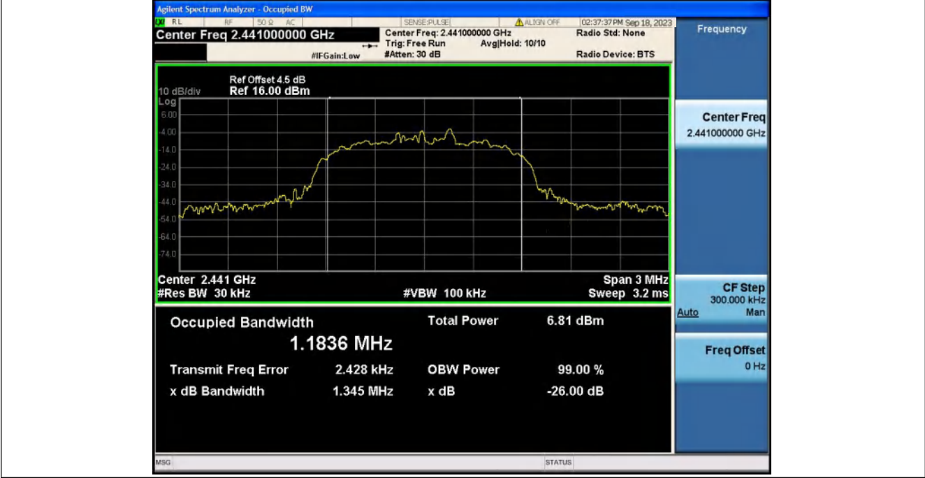
99%_Occupied_Bandwidth_NVNT_ANT1_3-DH5_2441
