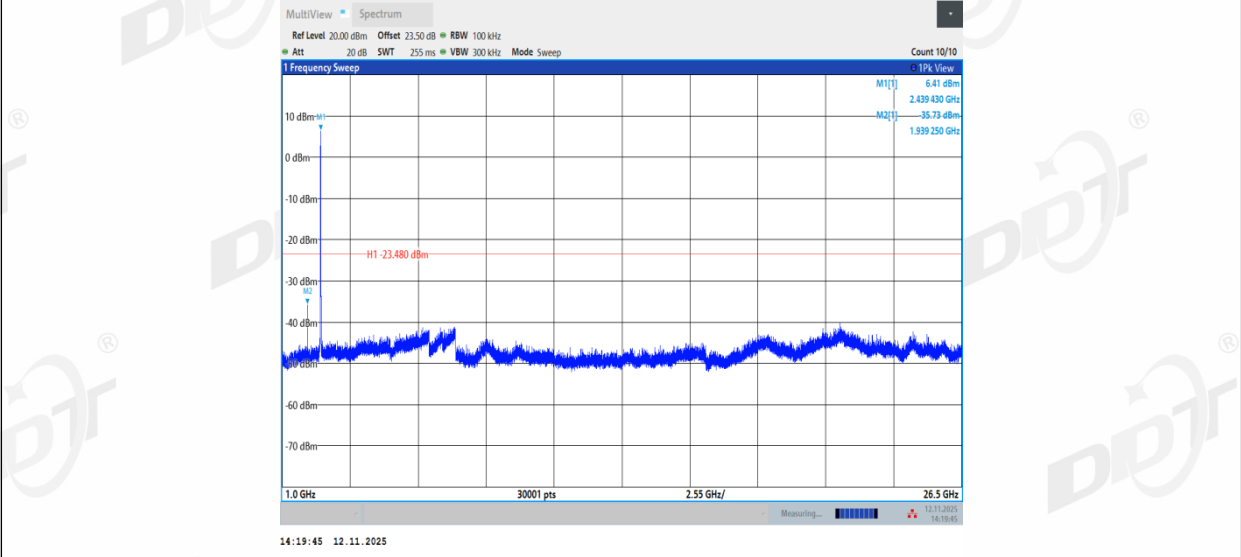
11G_Ant1_2462_0~Reference
