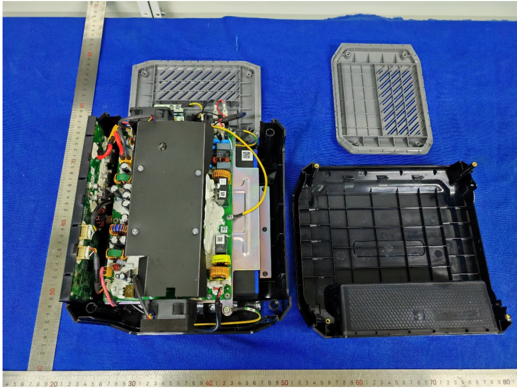
Disassembly view
