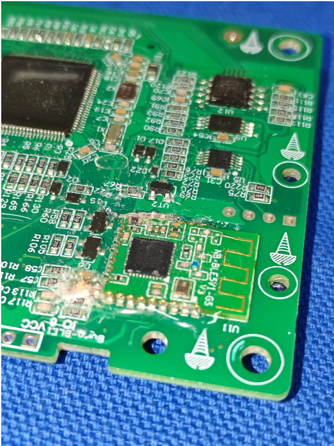
PCB bottom side without shielding
