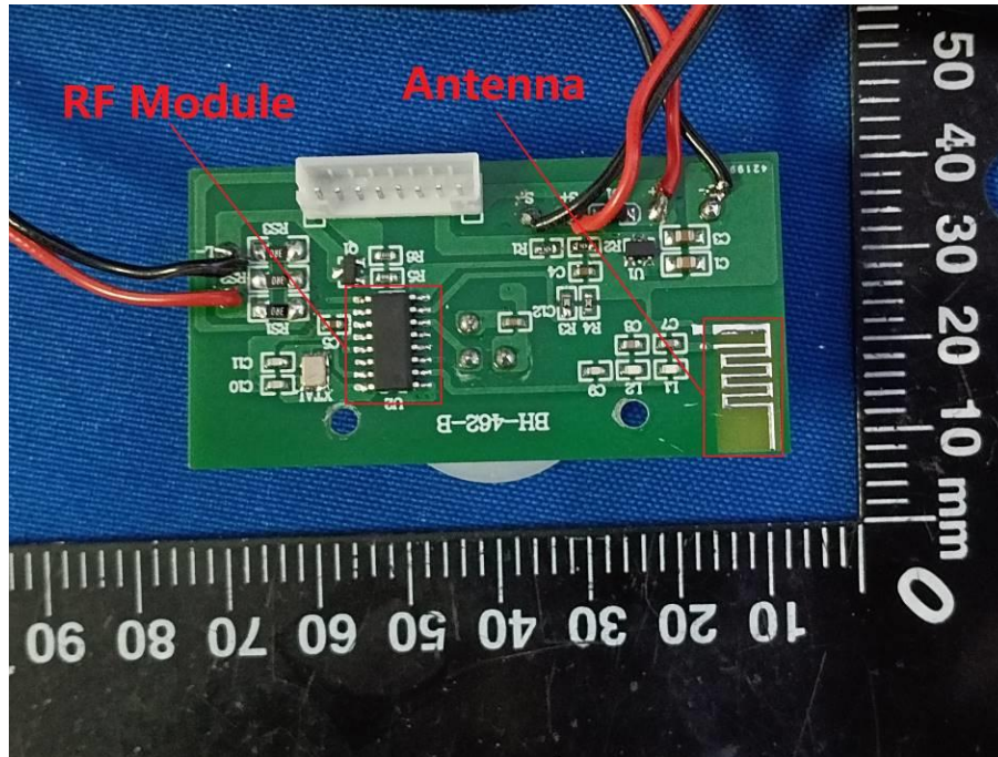
RF Module & Antenna Location-1
