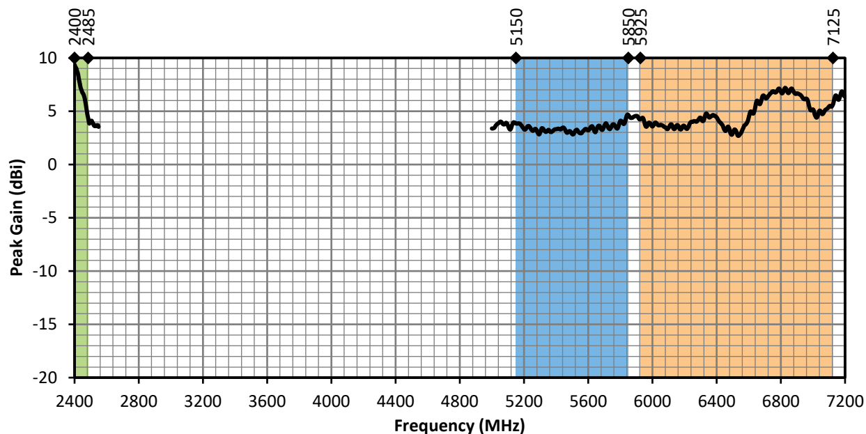
Figure 6. ANT-W63WS6-IPW1-ccc Peak Gain, Straight
