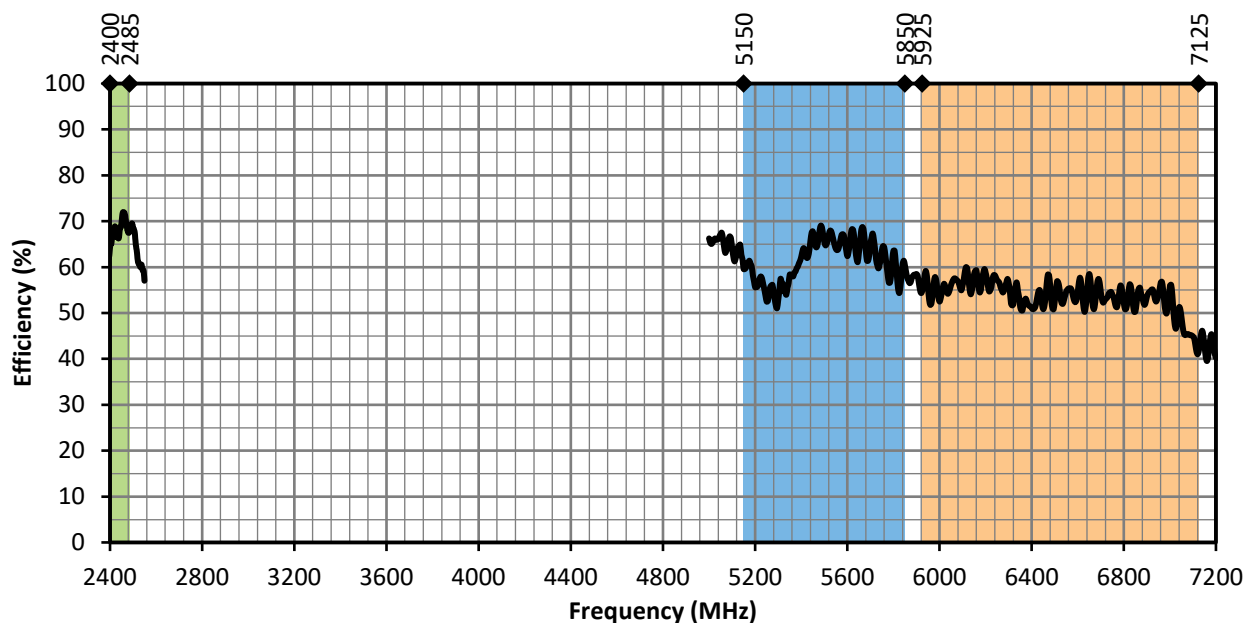
Figure 15. ANT-W63WS6-IPW1-ccc Antenna Efficiency, Edge-Bent
