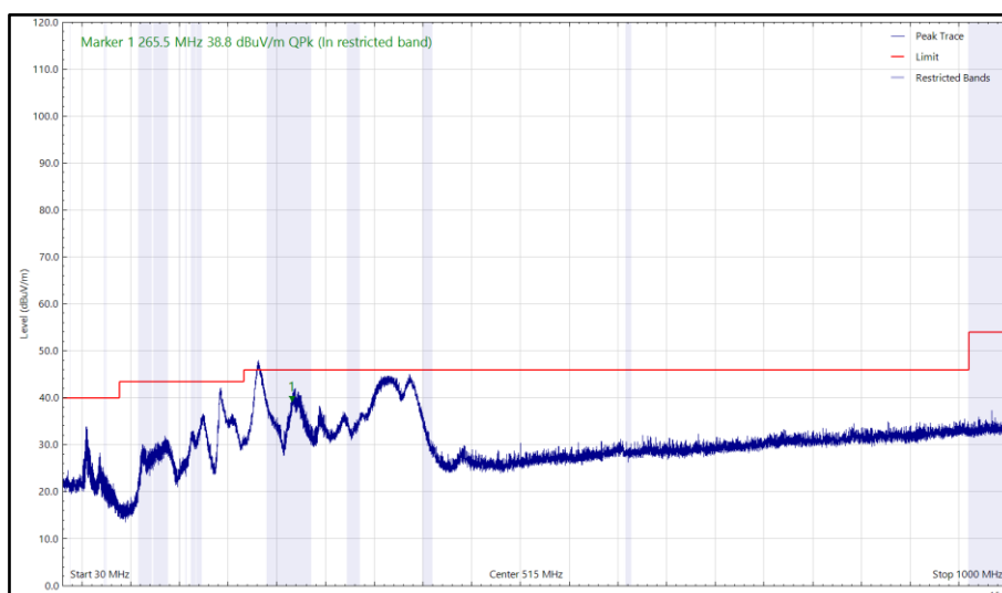
Figure 5 - 2412 MHz (CH1), 802.11b, 30 MHz to 1 GHz, Vertical (Peak)
