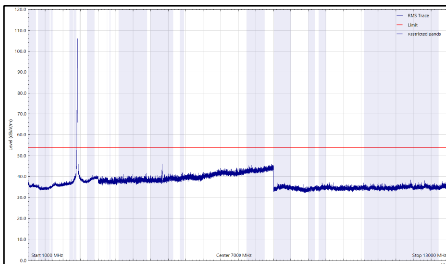
Figure 4 - 2412 MHz (CH1), 802.11b, 1 GHz to 13 GHz, Horizontal (rms)
