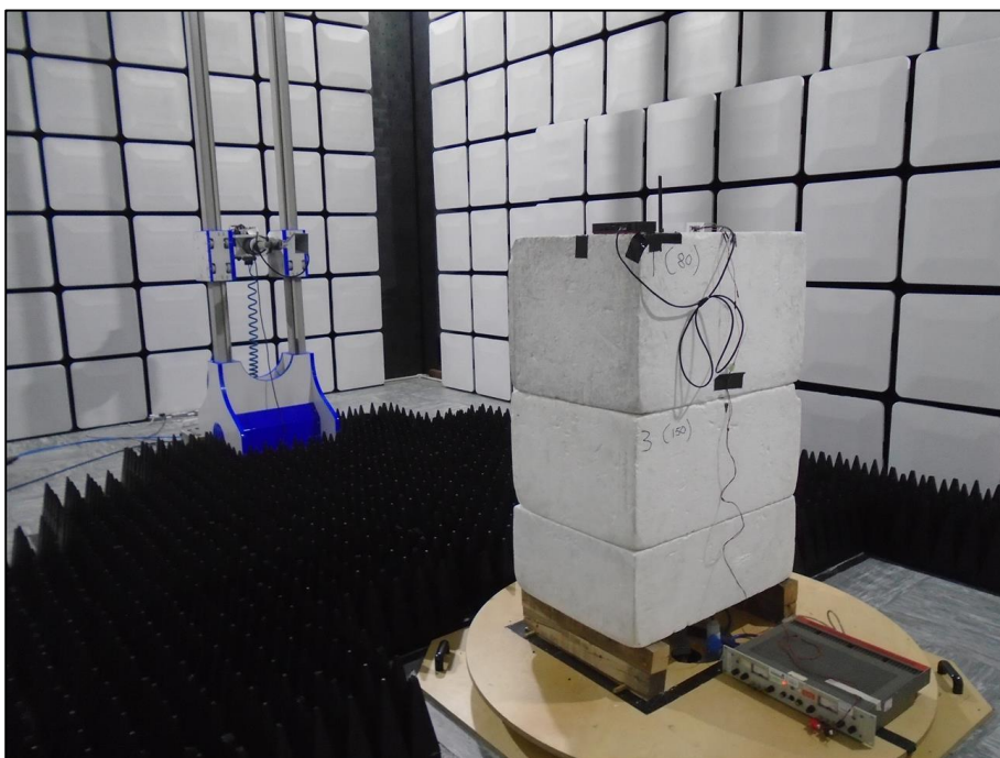
Figure 19 - Test Setup - 2.4 GHz WLAN External Antenna - 8 GHz to 13 GHz
