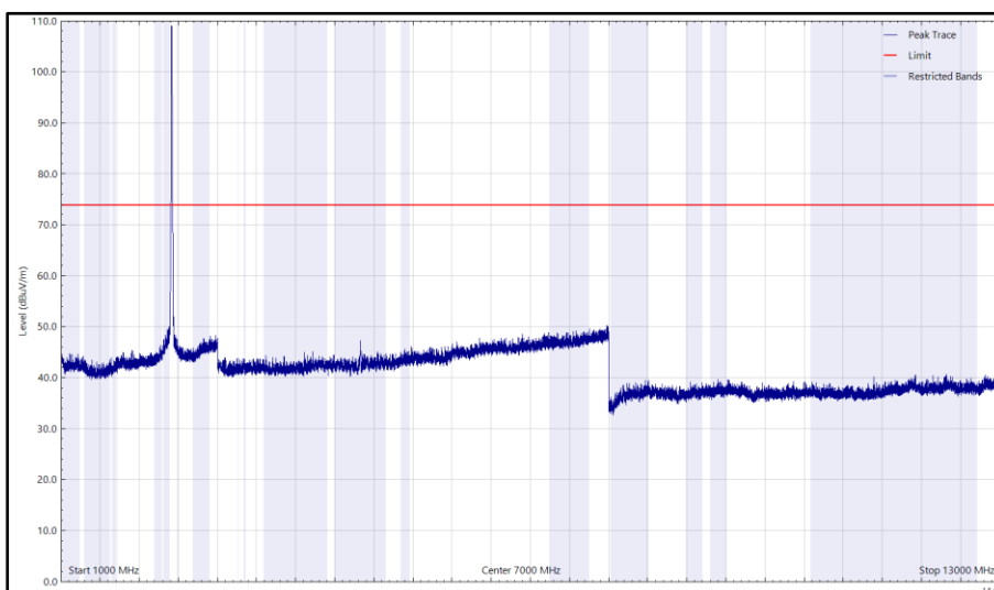
Figure 12 - 2412 MHz (CH1), 802.11b, 1 GHz to 13 GHz, Vertical (Peak)
