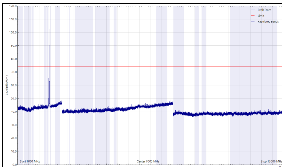
Figure 6 - 2412 MHz (CH1), 802.11b, 1 GHz to 13 GHz, Vertical (Peak)
