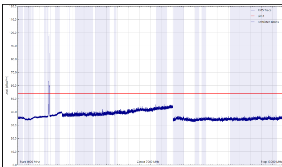
Figure 7 - 2412 MHz (CH1), 802.11b, 1 GHz to 13 GHz, Vertical (rms)
