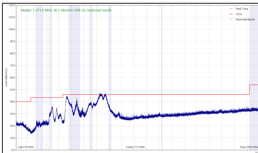
Figure 2 - 2412 MHz (CH1), 802.11b, 30 MHz to 1 GHz, Horizontal (Peak)
