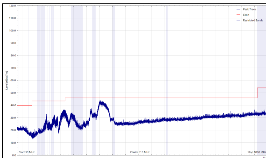
Figure 8 - 2412 MHz (CH1), 802.11b, 30 MHz to 1 GHz, Horizontal (Peak)
