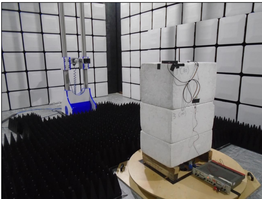
Figure 18 - Test Setup - 2.4 GHz WLAN External Antenna - 1 GHz to 8 GHz
