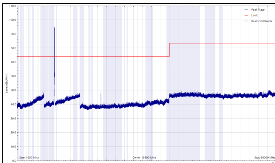
Figure 6 - U-NII-1 - 5180 MHz (CH36), HT20, 1 GHz to 30 GHz, Vertical (Peak)
