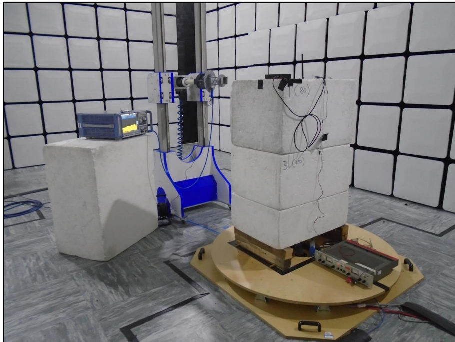
Figure 20 - Test setup, External Antenna - 18 GHz to 30 GHz
