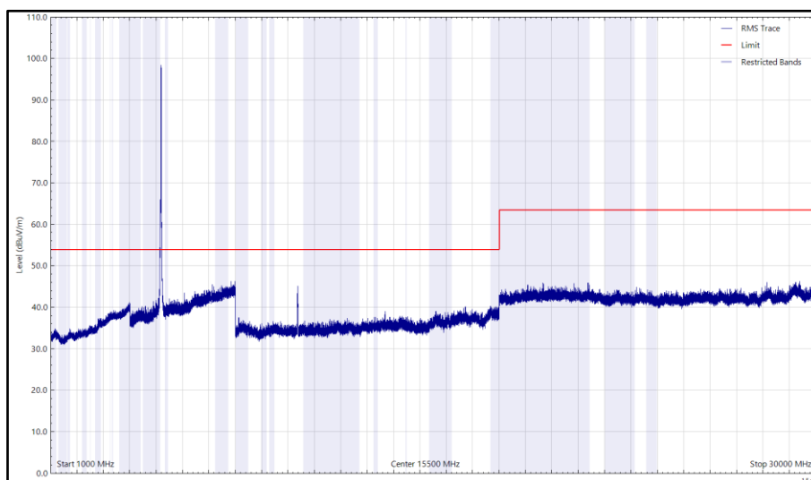
Figure 4 - U-NII-1 - 5180 MHz (CH36), HT20, 1 GHz to 30 GHz, Horizontal (rms)
