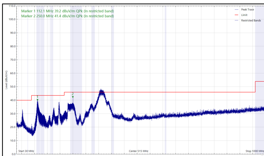
Figure 5 - U-NII-1 - 5180 MHz (CH36), HT20, 30 MHz to 1 GHz, Vertical (Peak)
