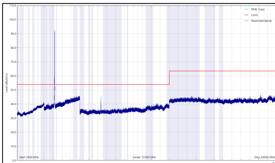
Figure 7 - U-NII-1 - 5180 MHz (CH36), HT20, 1 GHz to 30 GHz, Vertical (rms)
