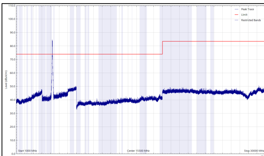
Figure 12 - 5190 MHz (CH36), HT40, 1 GHz to 30 GHz, Vertical (Peak)
