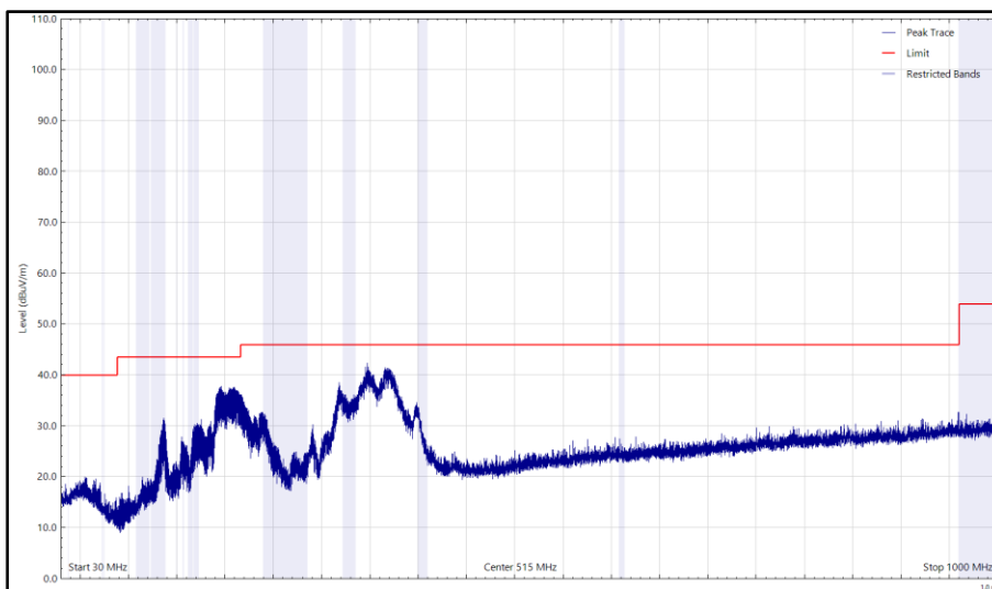
Figure 8 - 5190 MHz (CH36), HT40, 30 MHz to 1 GHz, Horizontal (Peak)
