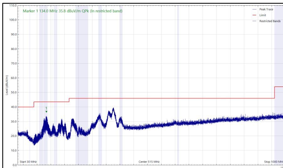
Figure 14 - CH1-802.11b-1Mbps_BLE-CH37_Ext, 2412 MHz_2402 MHz 30 MHz to 1 GHz, Horizontal (Peak)
