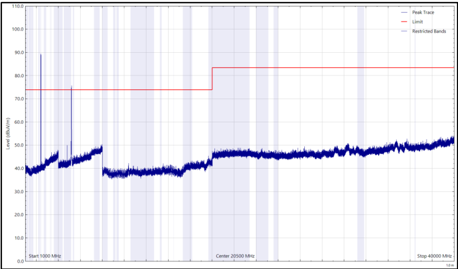
Figure 24 - CH38-HT40-MCS7_BLE-CH37, 5190 MHz_2402 MHz 1 GHz to 40 GHz, Vertical (Peak)
