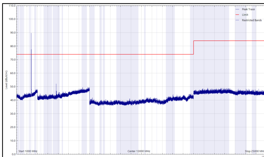
Figure 15 - CH1-802.11b-1Mbps_BLE-CH37_Ext, 2412 MHz_2402 MHz 1 GHz to 25 GHz, Horizontal (Peak)
