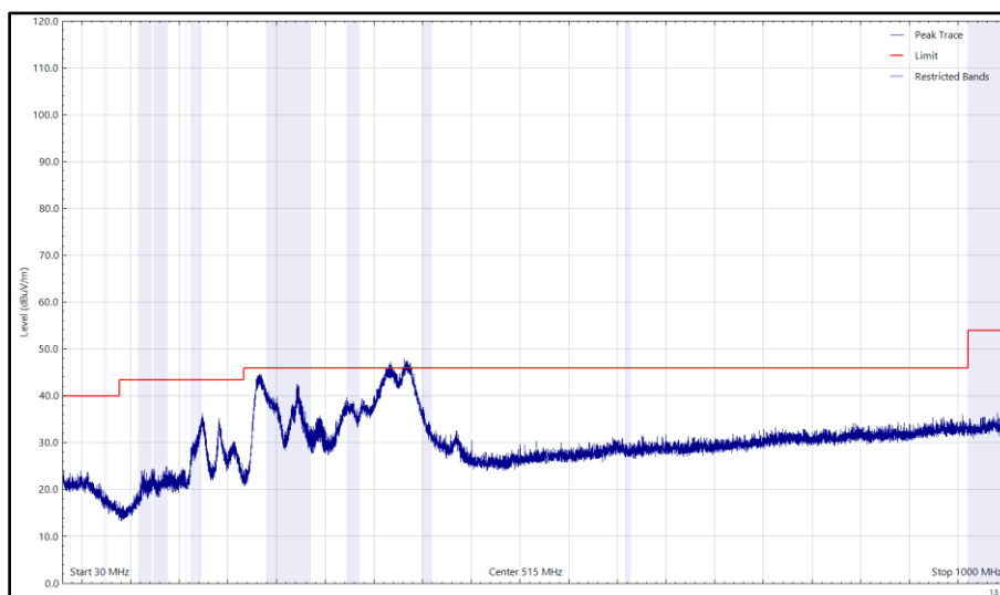
Figure 4 - 2402 MHz (CH37), BLE, 30 MHz to 1 GHz, Horizontal (Peak)
