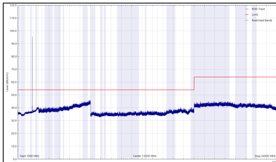
Figure 9 - 2402 MHz (CH37), BLE, 1 GHz to 26 GHz, Vertical (rms)
