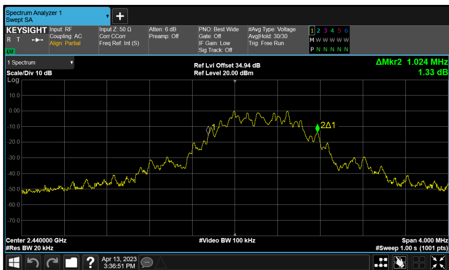
Figure 24 - P7 (A) 2440 MHz (CH17) 99% Bandwidth
