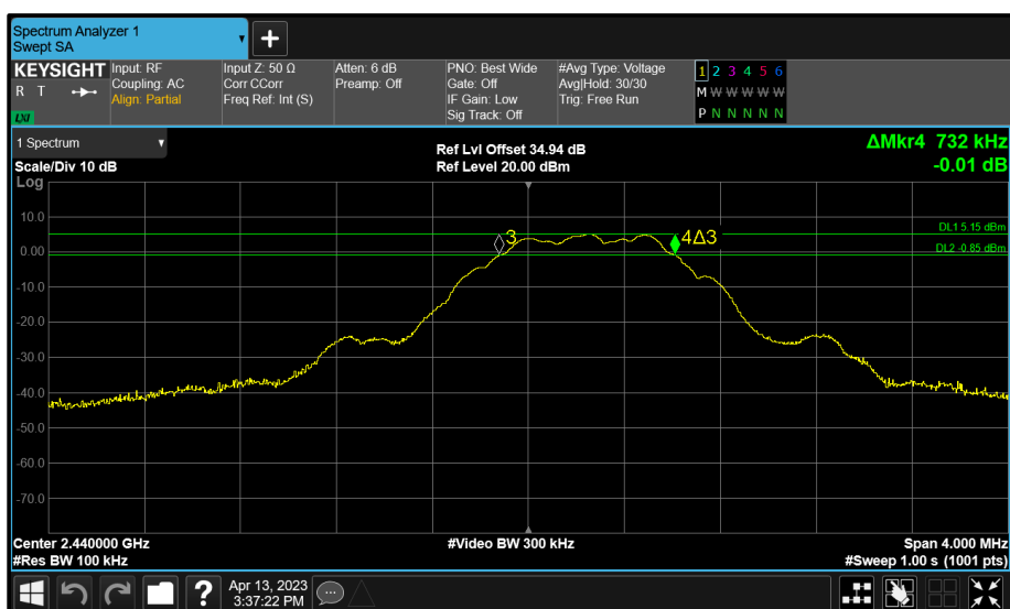
Figure 25 - P7 (A) 2440 MHz (CH17) 6 dB Bandwidth
