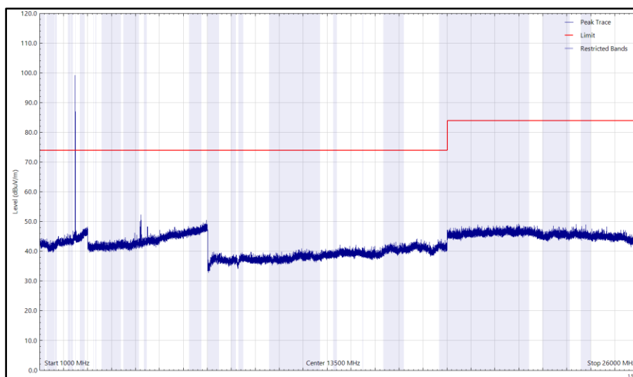
Figure 17 - 2480 MHz (CH39), BLE, 1 GHz to 26 GHz, Horizontal (Peak)
