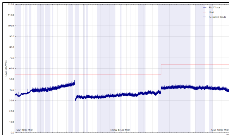
Figure 15 - 2440 MHz (CH17), BLE, 1 GHz to 26 GHz, Vertical (rms)
