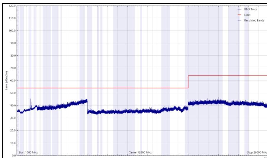
Figure 6 - 2402 MHz (CH37), BLE, 1 GHz to 26 GHz, Horizontal (rms)
