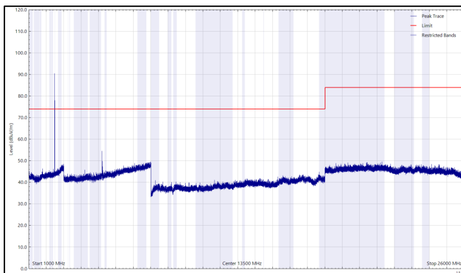
Figure 20 - 2480 MHz (CH39), BLE, 1 GHz to 26 GHz, Vertical (Peak)
