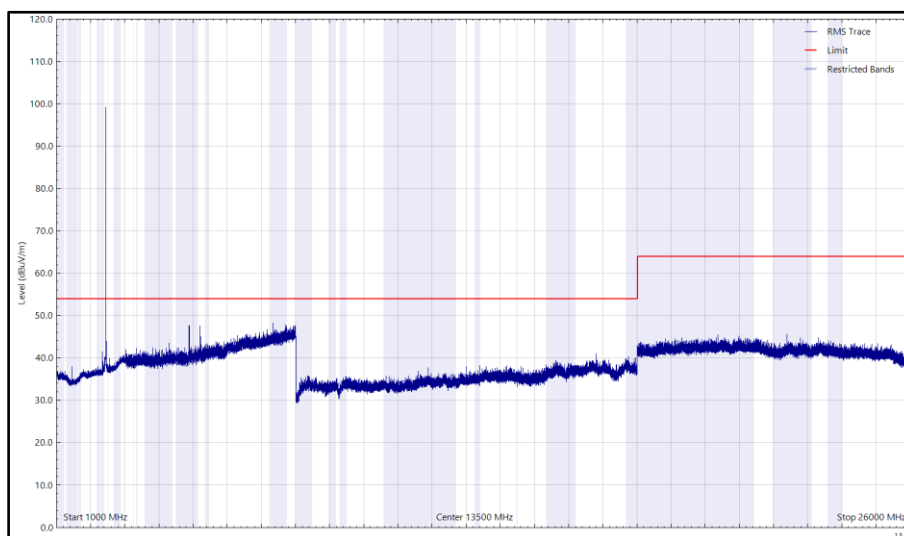
Figure 12 - 2440 MHz (CH17), BLE, 1 GHz to 26 GHz, Horizontal (rms)
