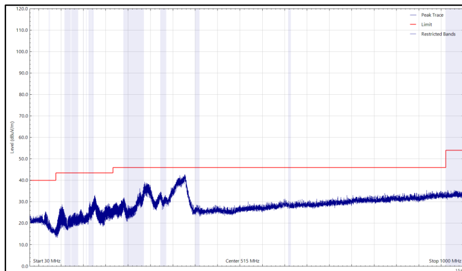
Figure 19 - 2480 MHz (CH39), BLE, 30 MHz to 1 GHz, Vertical (Peak)
