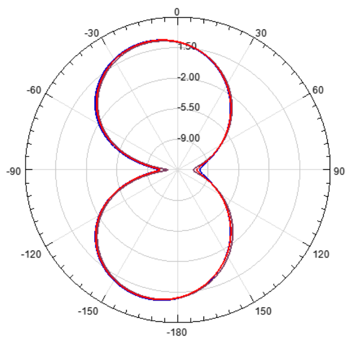
Radiation Pattern YO
