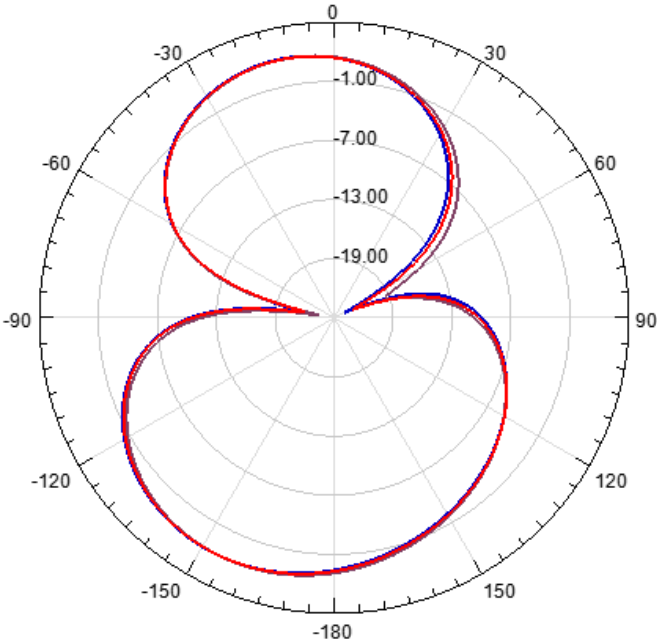
Radiation Pattern XOY
