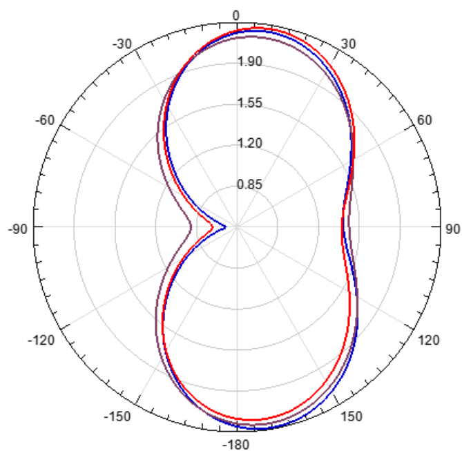
Radiation Pattern XOZ
