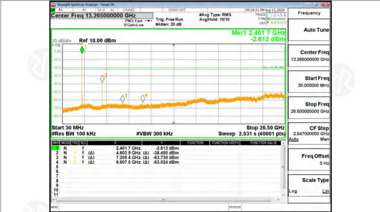
Tx. Spurious NVNT 1-DH5 2402MHz Ant1 Emission
