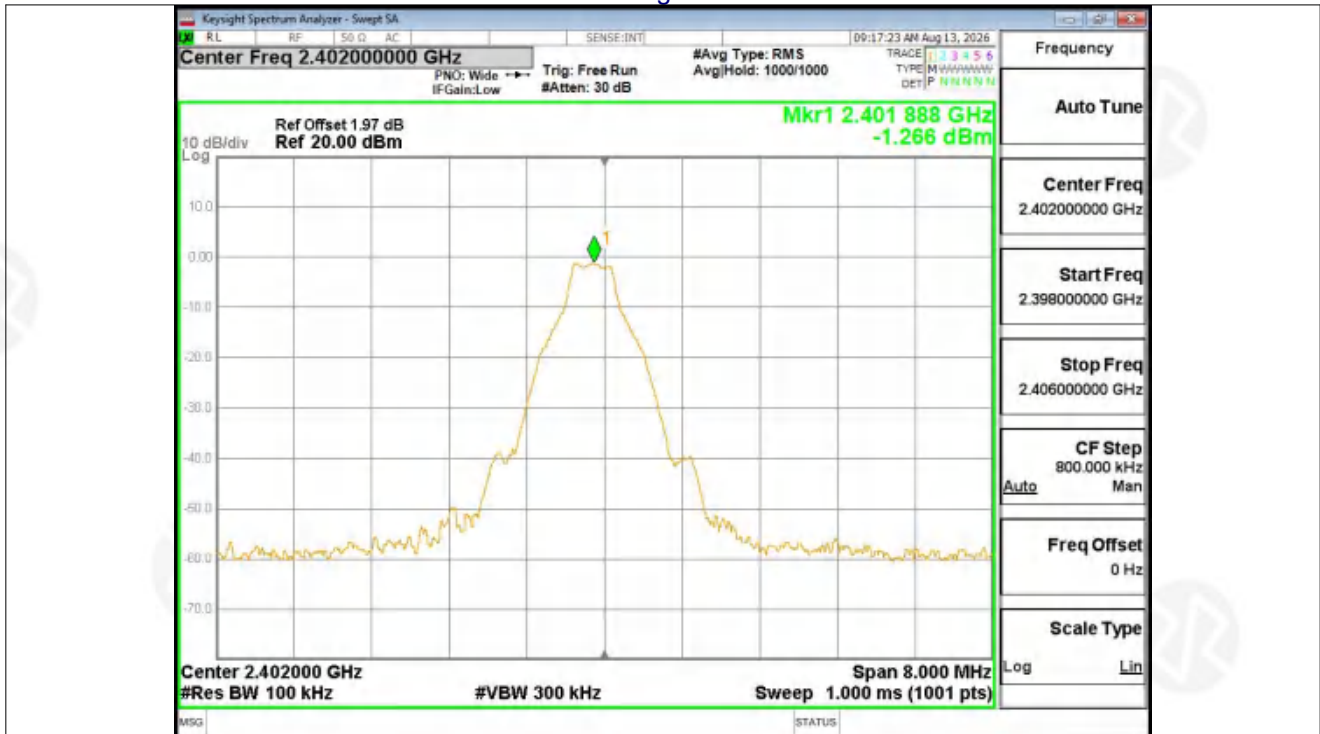
Band Edge NVNT 1-DH5 2402MHz Ant1 No-Hopping Ref
