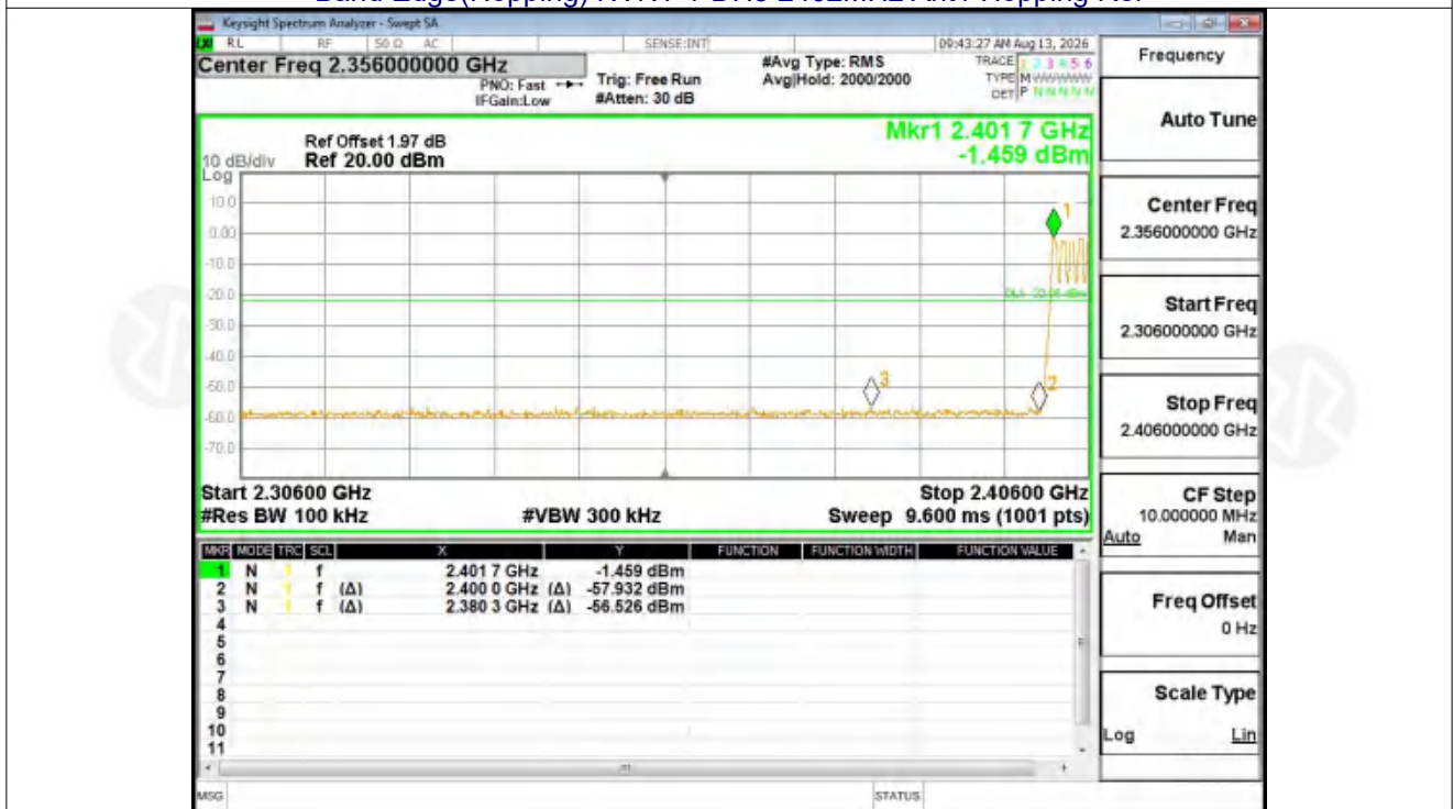
Band Edge(Hopping) NVNT 1-DH5 2402MHz Ant1 Hopping Emission
