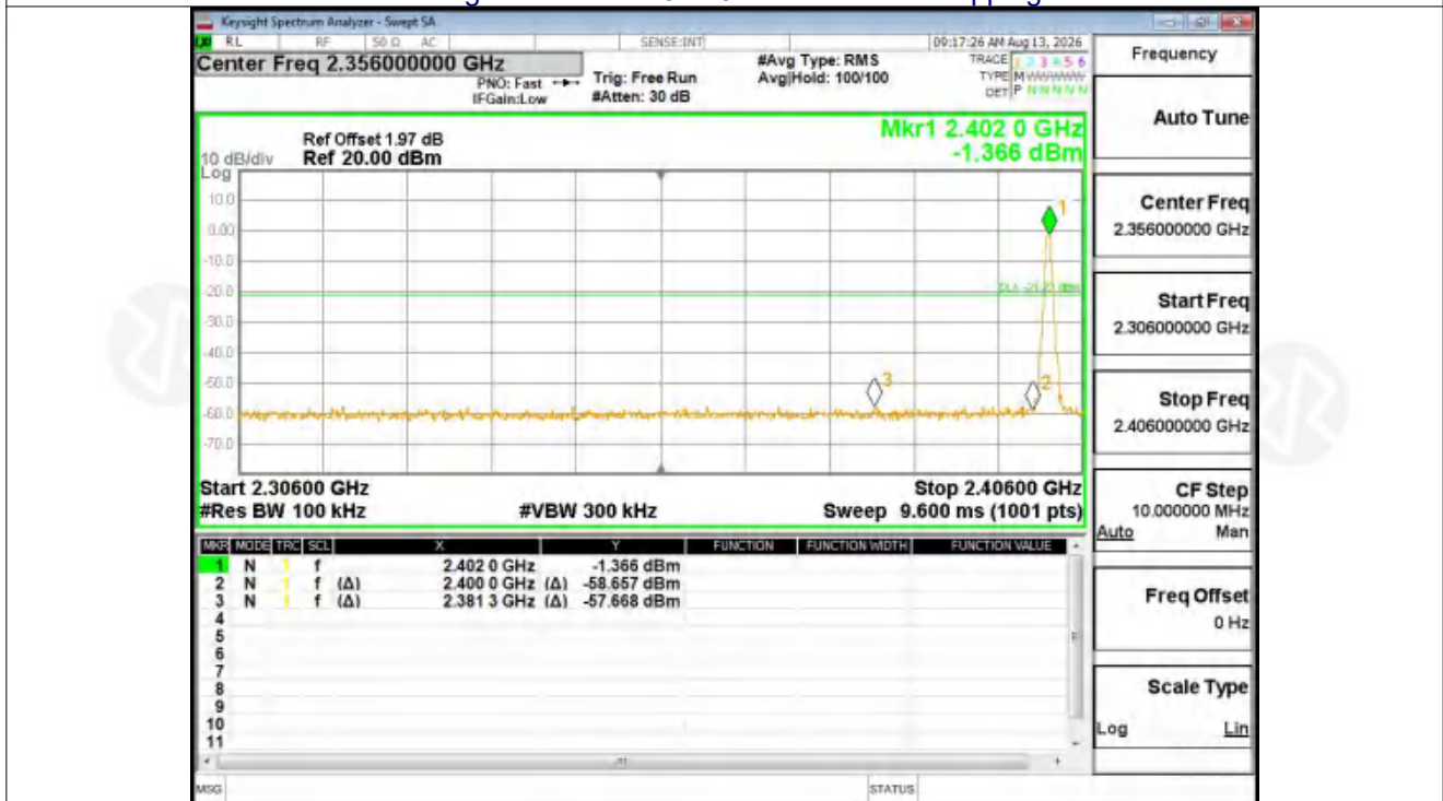
Band Edge NVNT 1-DH5 2402MHz Ant1 No-Hopping Emission
