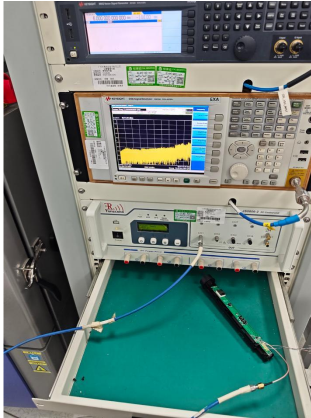
Conducted Emission Test View
