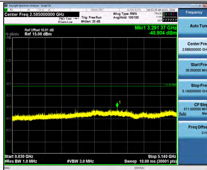
11AX20SISO_Ant3_5180_5360~27000
