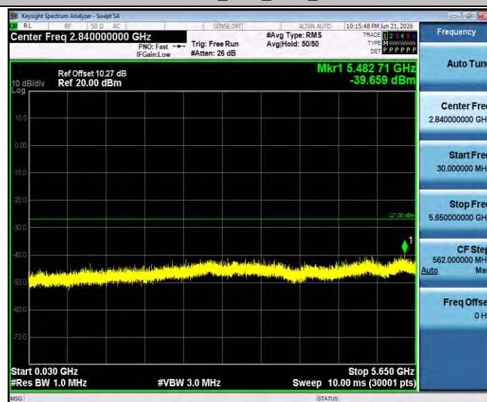
11AC40SISO_Ant3_5795_30~5650
