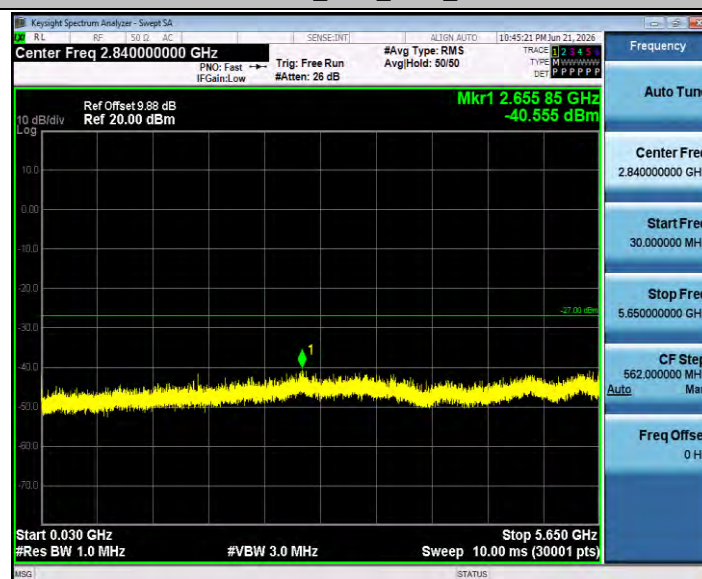
11AX40SISO_Ant3_5755_30~5650
