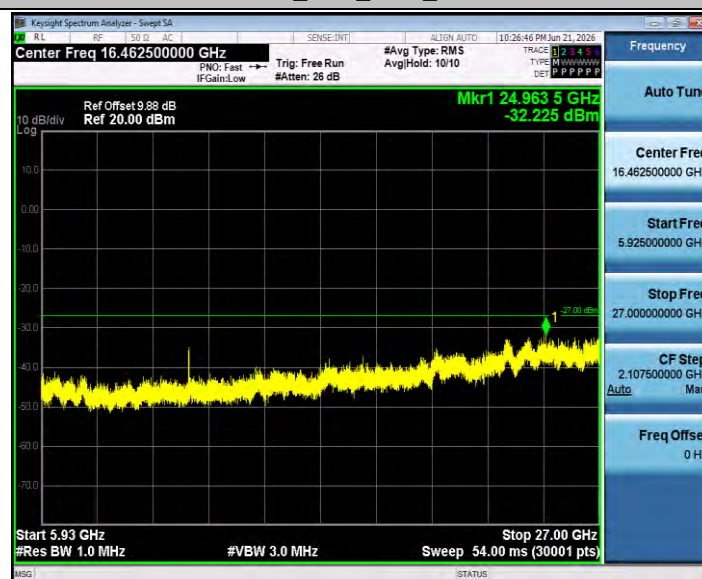
11AX20SISO_Ant3_5745_5925~27000
