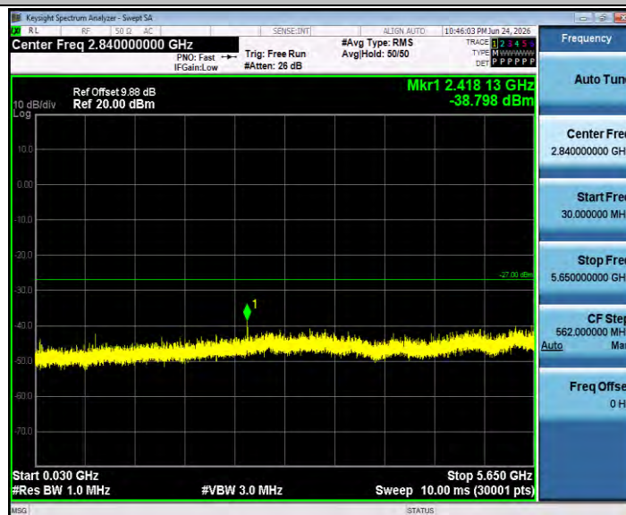
11AX40SISO_Ant3_5755_30~5650
