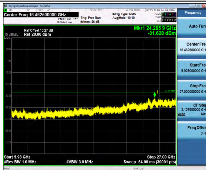
11N20SISO_Ant3_5785_5925~27000
