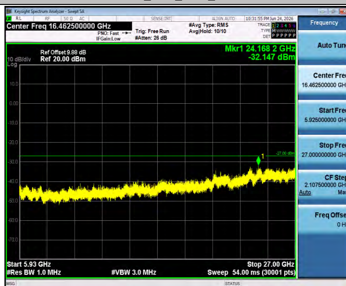
11AX20SISO_Ant3_5745_5925~27000
