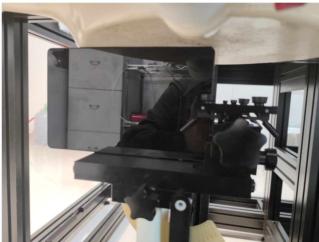
WLAN ANT0 Body Right Setup Photo (0 mm)
