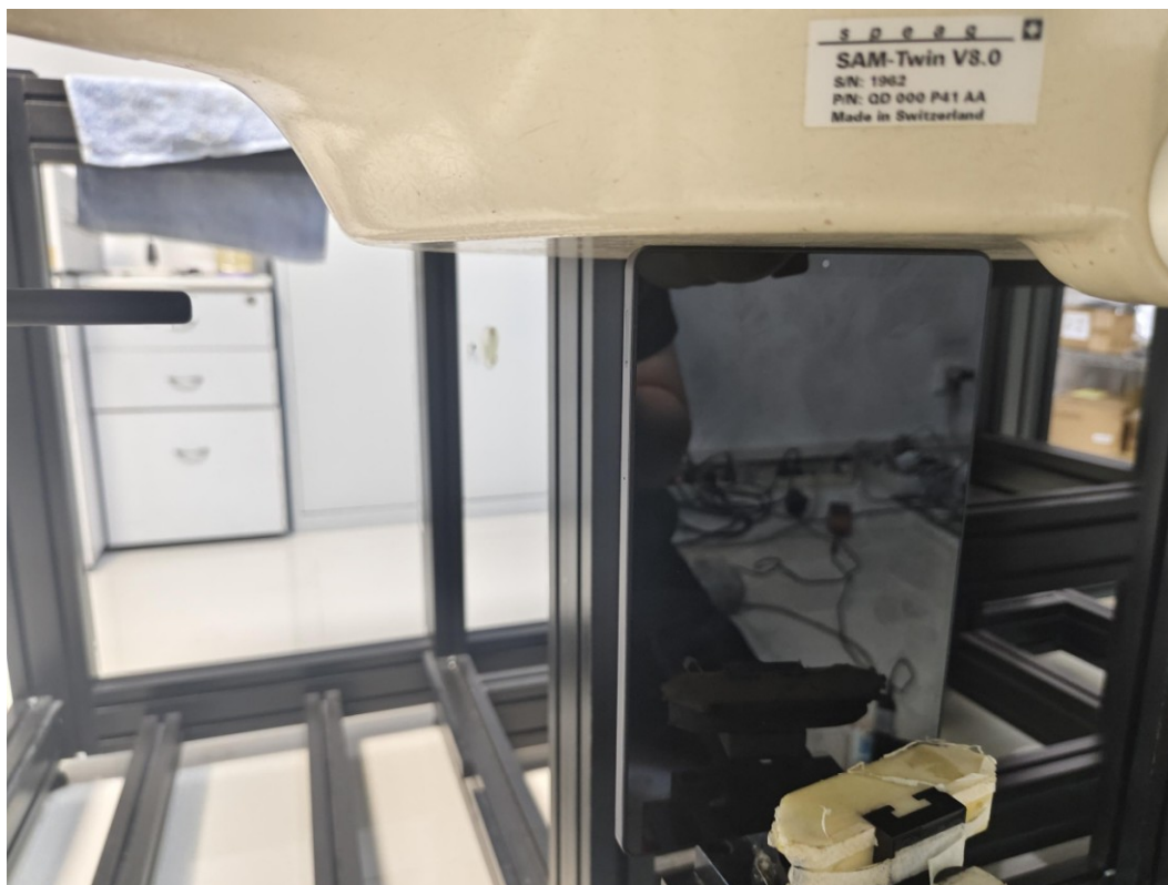
WLAN ANT1 Body Top Setup Photo (0 mm)
