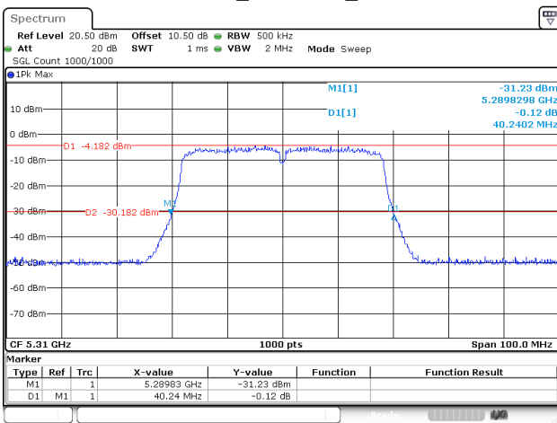
802.11ac40_5310MHz_Chain 1
