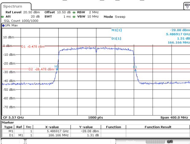
802.11ax160_5570MHz_RU_FULL_Chain 0
