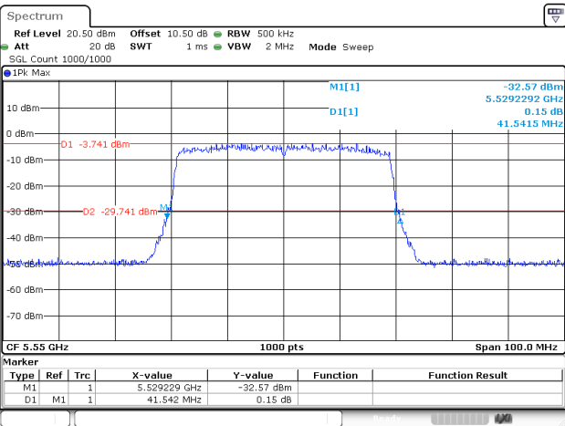
802.11ax40_5550MHz_RU_FULL_Chain 1
