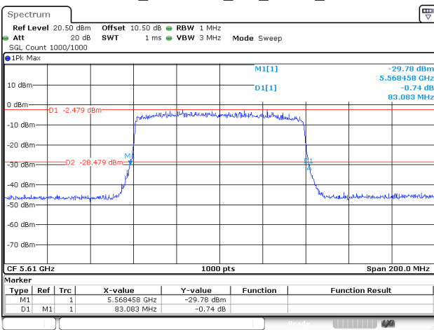
802.11ax80_5610MHz_RU_FULL_Chain 1
