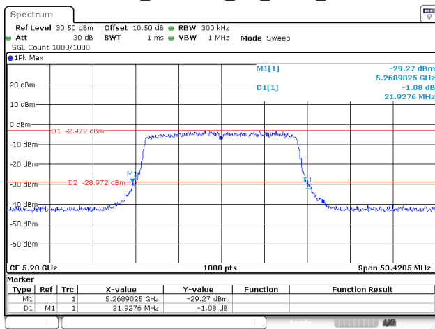
802.11ax20_5280MHz_RU_FULL_Chain 0
