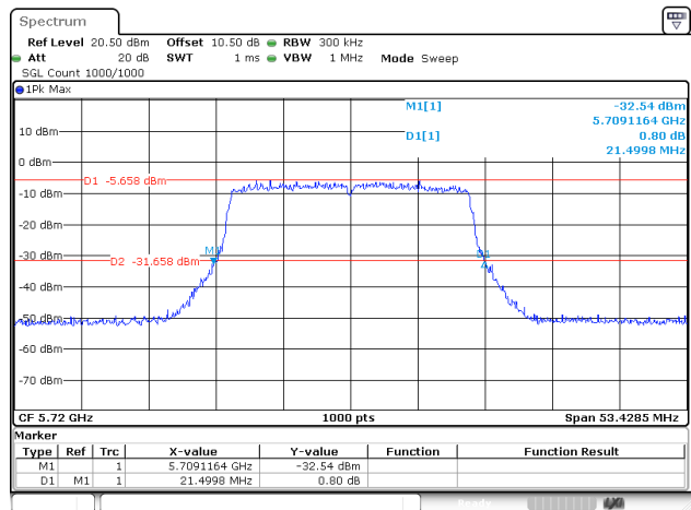
802.11ax20_5720MHz_RU_FULL_Chain 1
