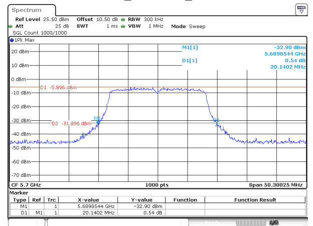
802.11a_5700MHz_Chain 1
