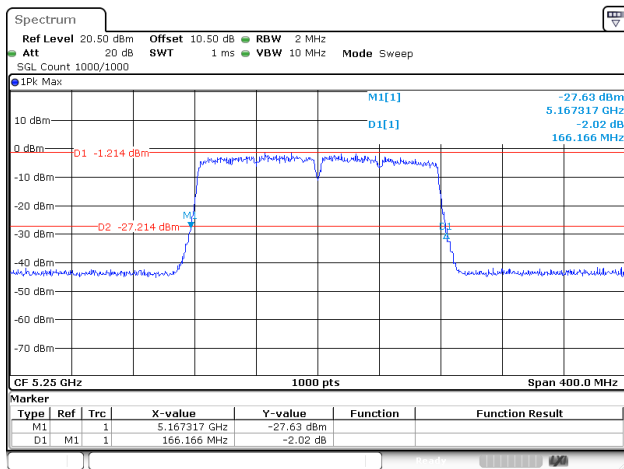
802.11ac160_5250MHz_RU_FULL_Chain 1
