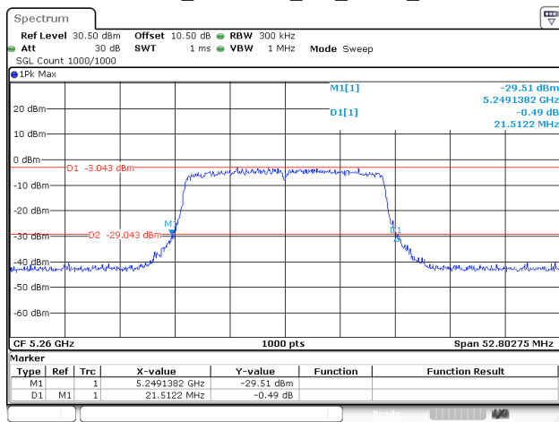
802.11ax20_5260MHz_RU_FULL_Chain 0
