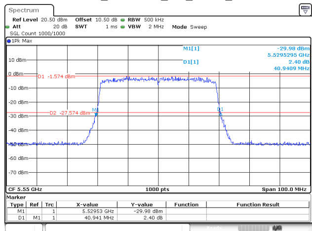
802.11ax40_5550MHz_RU_FULL_Chain 0
