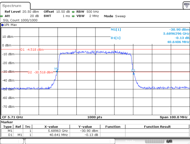
802.11ax40_5710MHz_RU_FULL_Chain 1
