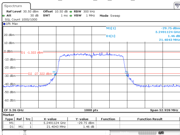
802.11ax20_5260MHz_RU_FULL_Chain 1
