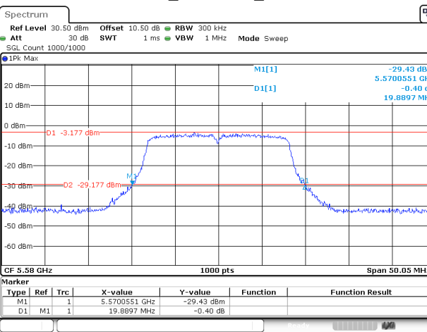
802.11a_5580MHz_Chain 1
