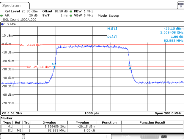
802.11ax80_5610MHz_RU_FULL_Chain 0
