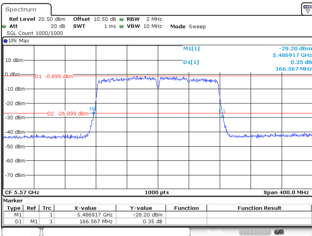
802.11ac160_5570MHz_RU_FULL_Chain 0
