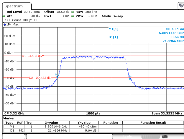
802.11ax20_5320MHz_RU_FULL_Chain 0
