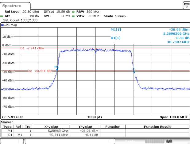
802.11ax40_5310MHz_RU_FULL_Chain 0
