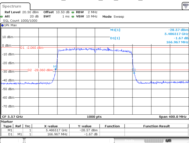
802.11ax160_5570MHz_RU_FULL_Chain 1
