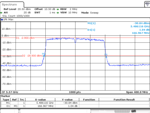
802.11ac160_5570MHz_RU_FULL_Chain 1
