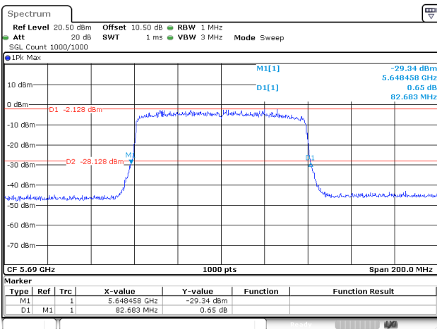
802.11ax80_5690MHz_RU_FULL_Chain 0
