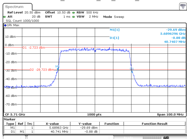
802.11ax40_5710MHz_RU_FULL_Chain 0
