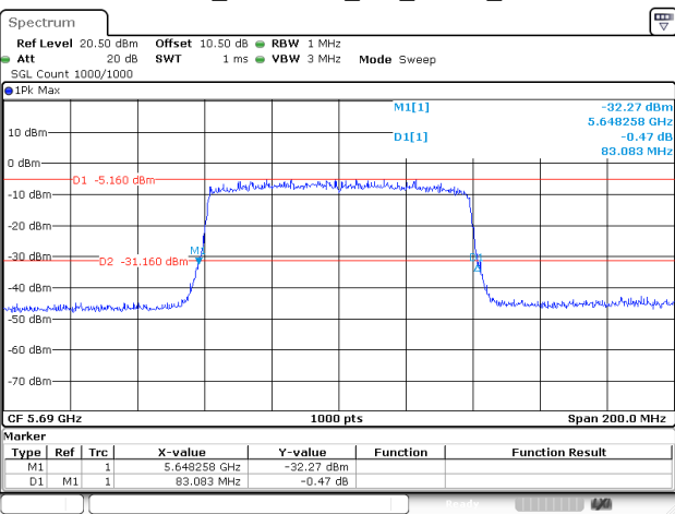
802.11ax80_5690MHz_RU_FULL_Chain 1
