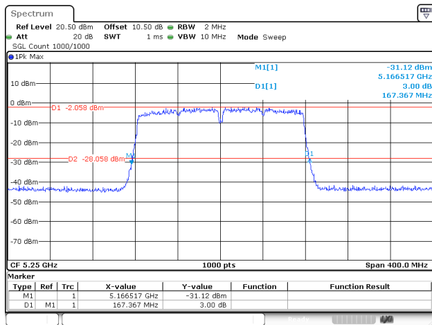
802.11ac160_5250MHz_RU_FULL_Chain 0
