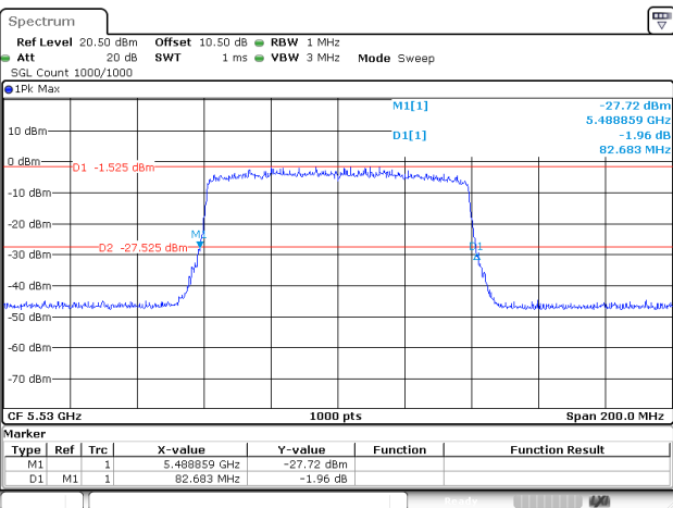
802.11ax80_5530MHz_RU_FULL_Chain 1
