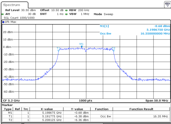
802.11a_5200MHz_Chain 1
