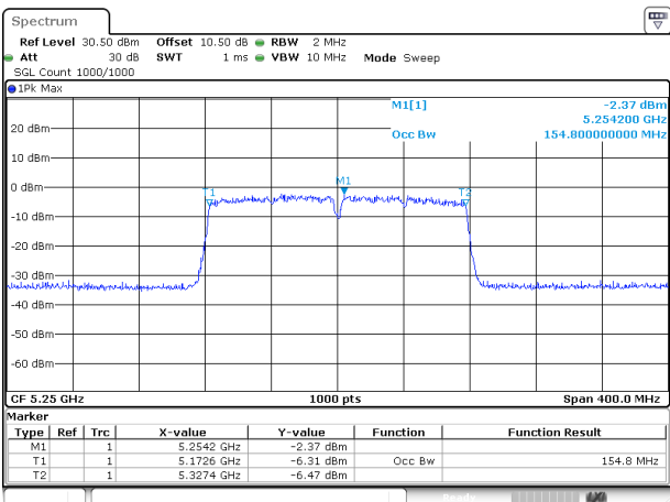
802.11ac160_5250MHz_RU_FULL_Chain 1
