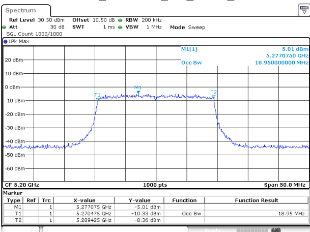
802.11ax20_5280MHz_RU_FULL_Chain 0
