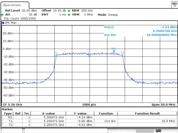
802.11ax20_5260MHz_RU_FULL_Chain 1
