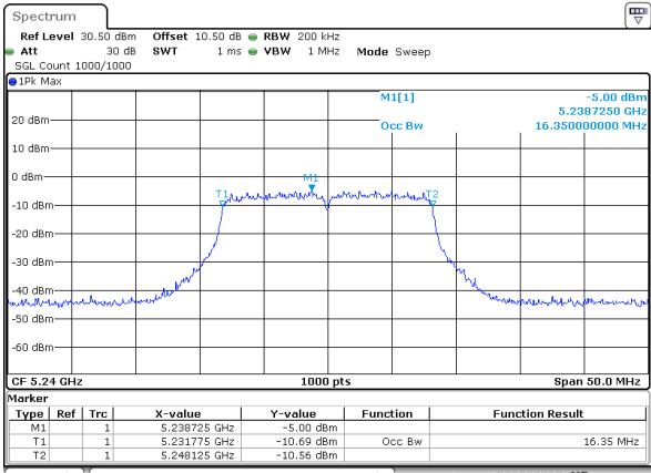
802.11a_5240MHz_Chain 0
