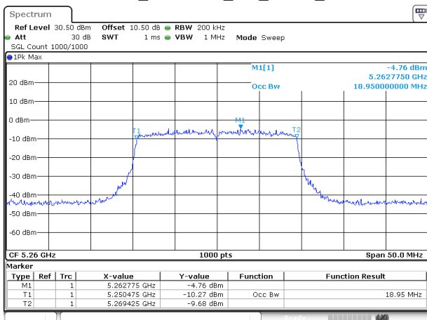
802.11ax20_5260MHz_RU_FULL_Chain 0
