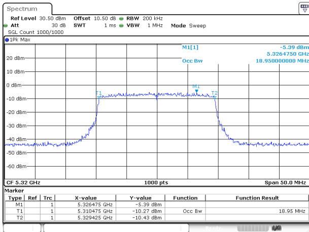
802.11ax20_5320MHz_RU_FULL_Chain 0
