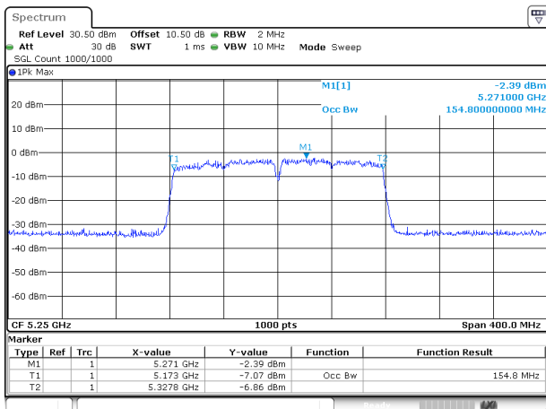
802.11ac160_5250MHz_RU_FULL_Chain 0
