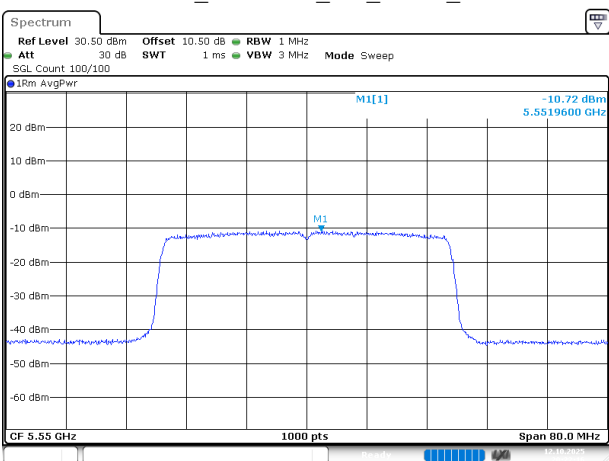
802.11ax40_5550MHz_RU_FULL_Chain 0
