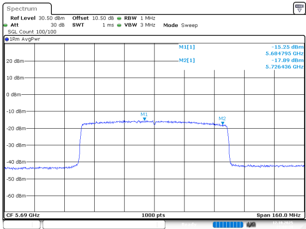
802.11ax80_5690MHz_RU_FULL_Chain 0
