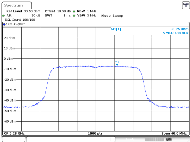
802.11ax20_5280MHz_RU_FULL_Chain 1
