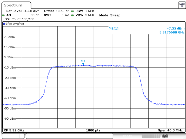
802.11ax20_5320MHz_RU_FULL_Chain 0
