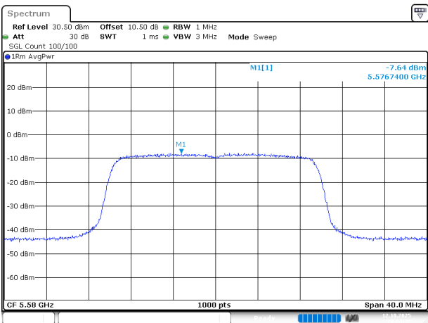
802.11ax20_5580MHz_RU_FULL_Chain 0
