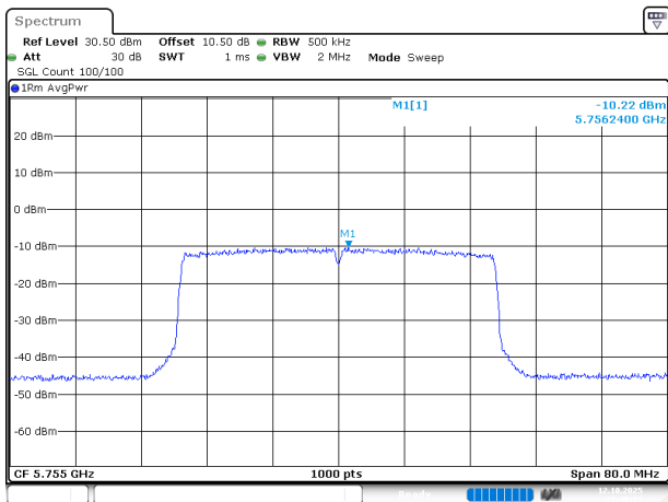
802.11ax40_5755MHz_RU_FULL_Chain 0
