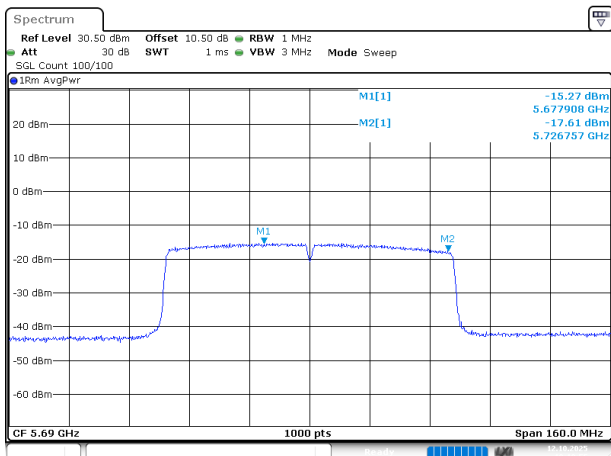
802.11ac80_5690MHz_Chain 0
