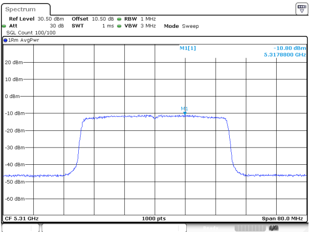
802.11ax40_5310MHz_RU_FULL_Chain 0
