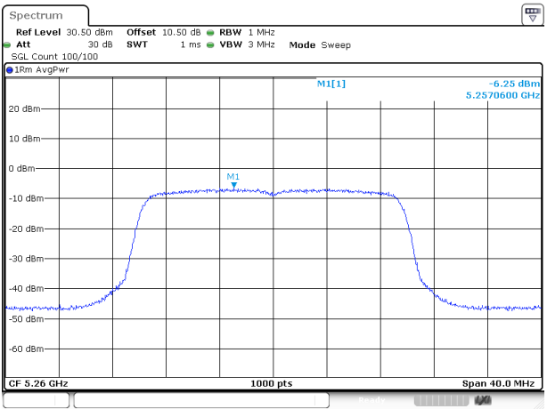
802.11ax20_5260MHz_RU_FULL_Chain 1
