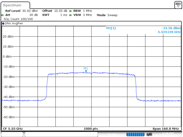
802.11ax80_5530MHz_RU_FULL_Chain 1
