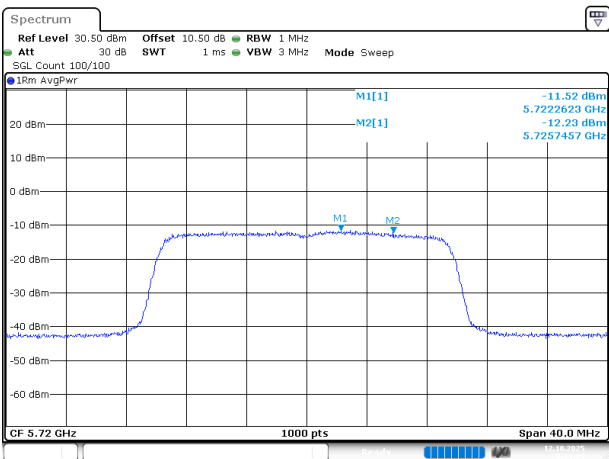
802.11ax20_5720MHz_RU_FULL_Chain 1
