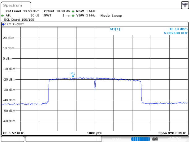
802.11ax160_5570MHz_RU_FULL_Chain 1
