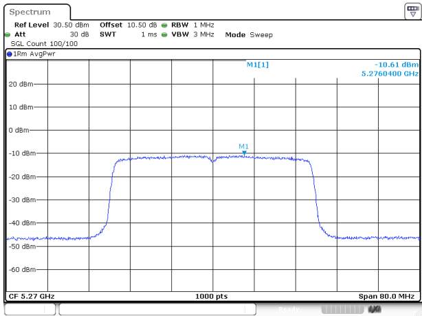
802.11ax40_5270MHz_RU_FULL_Chain 1
