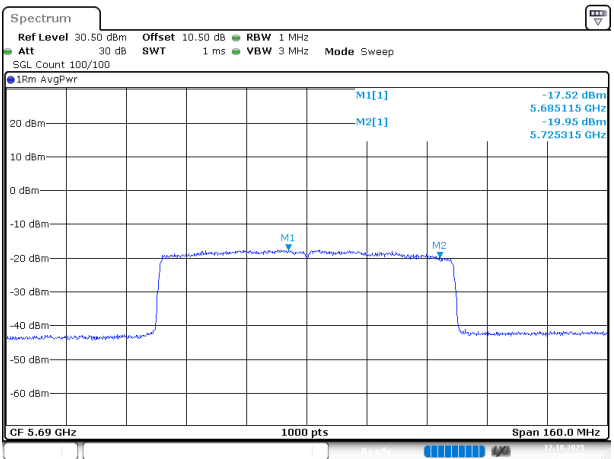
802.11ax80_5690MHz_RU_FULL_Chain 1
