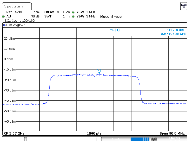
802.11ax40_5670MHz_RU_FULL_Chain 1
