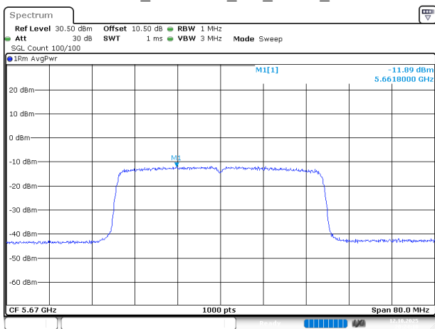
802.11ax40_5670MHz_RU_FULL_Chain 0
