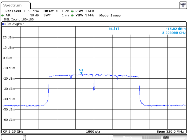
802.11ac160_5250MHz_RU_FULL_Chain 1
