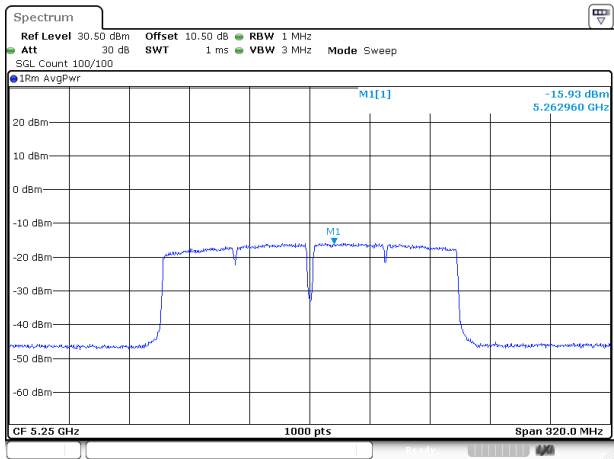
802.11ac160_5250MHz_RU_FULL_Chain 0
