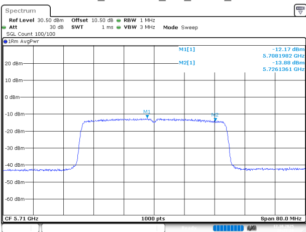
802.11ax40_5710MHz_RU_FULL_Chain 0
