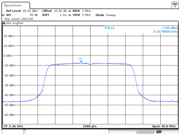
802.11ax20_5260MHz_RU_FULL_Chain 0
