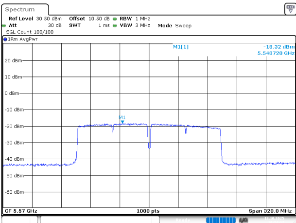
802.11ac160_5570MHz_RU_FULL_Chain 1
