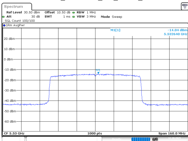
802.11ax80_5530MHz_RU_FULL_Chain 0
