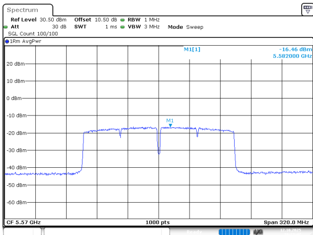
802.11ac160_5570MHz_RU_FULL_Chain 0
