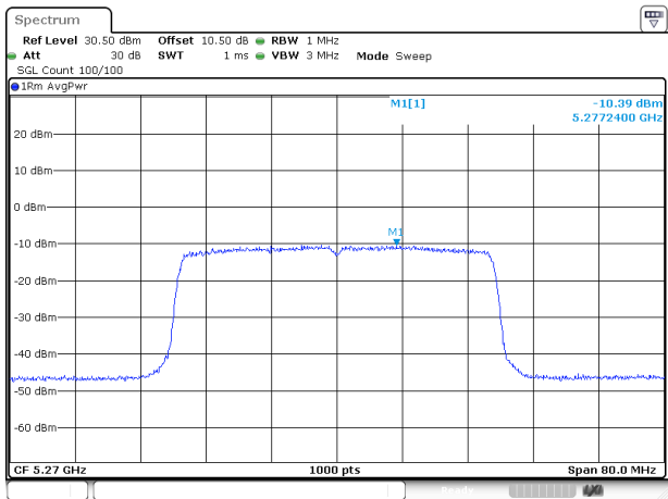
802.11ax40_5270MHz_RU_FULL_Chain 0
