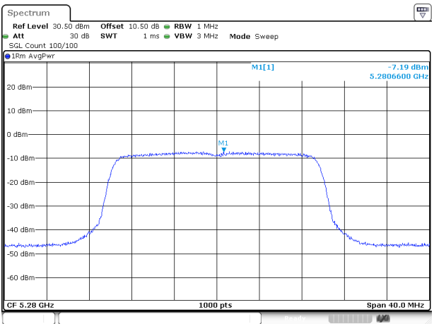
802.11ax20_5280MHz_RU_FULL_Chain 0
