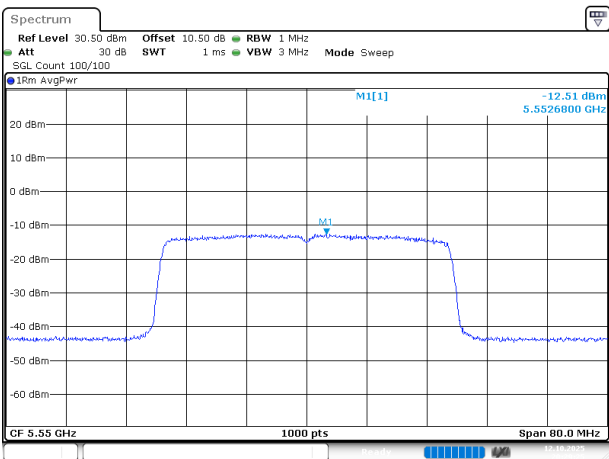
802.11ax40_5550MHz_RU_FULL_Chain 1
