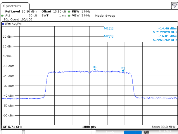
802.11ax40_5710MHz_RU_FULL_Chain 1
