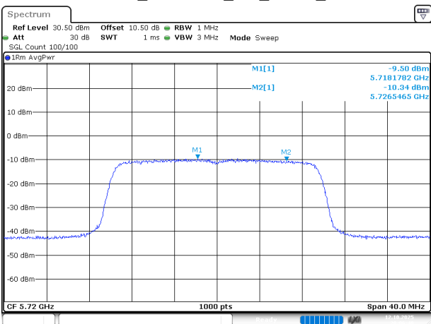
802.11ax20_5720MHz_RU_FULL_Chain 0
