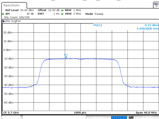
802.11ax20_5700MHz_RU_FULL_Chain 0
