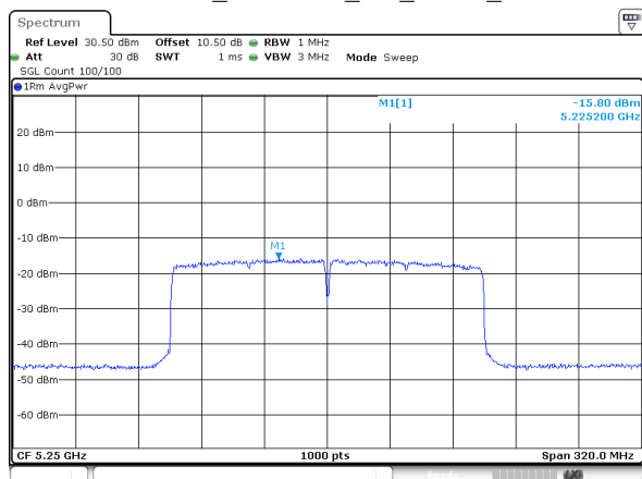
802.11ax160_5250MHz_RU_FULL_Chain 1
