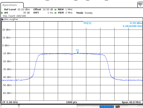
802.11ax20_5580MHz_RU_FULL_Chain 1
