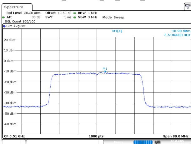
802.11ax40_5510MHz_RU_FULL_Chain 0
