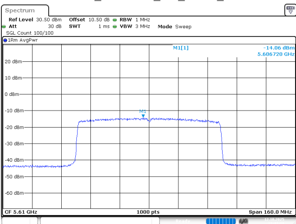
802.11ax80_5610MHz_RU_FULL_Chain 0
