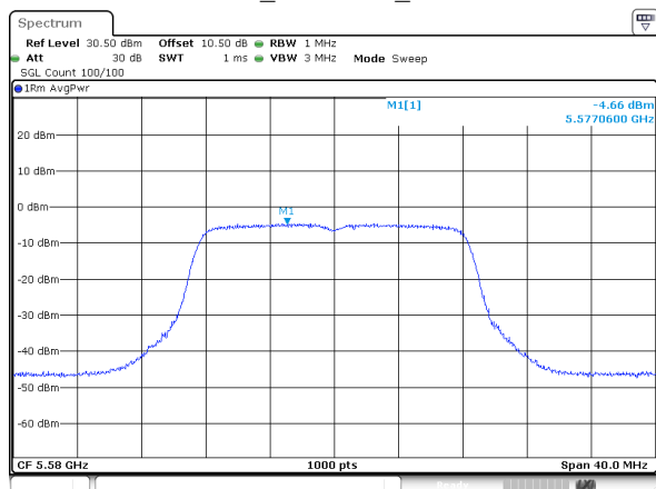
802.11a_5580MHz_Chain 0
