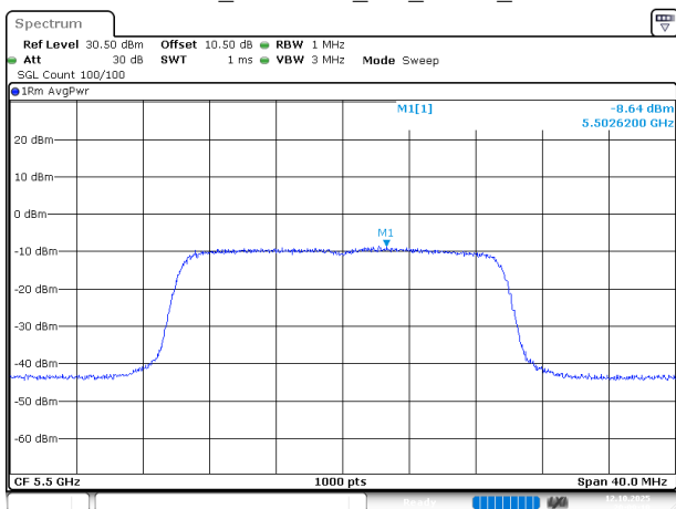
802.11ax20_5500MHz_RU_FULL_Chain 1
