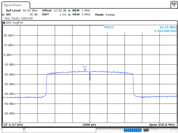
802.11ax160_5570MHz_RU_FULL_Chain 0
