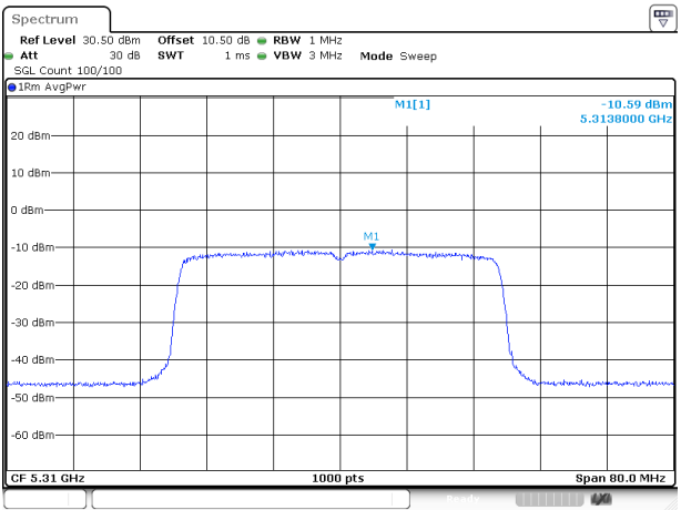
802.11ax40_5310MHz_RU_FULL_Chain 1
