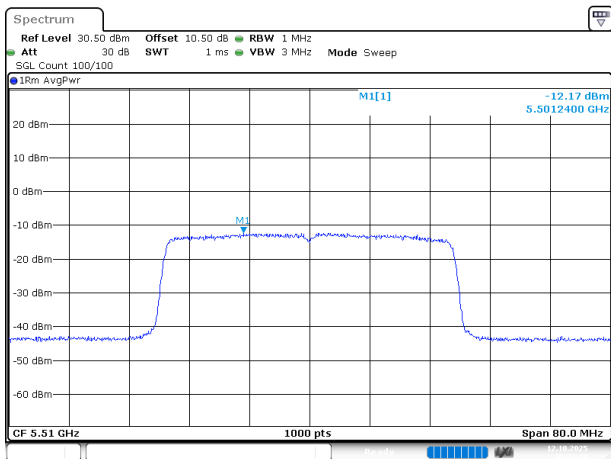
802.11ax40_5510MHz_RU_FULL_Chain 1
