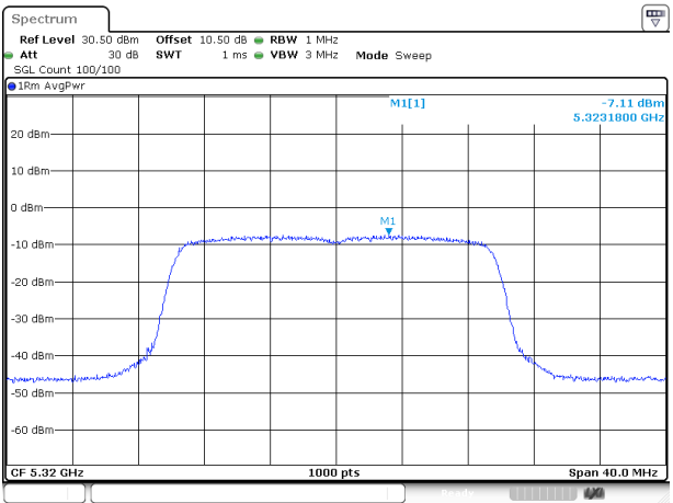
802.11ax20_5320MHz_RU_FULL_Chain 1
