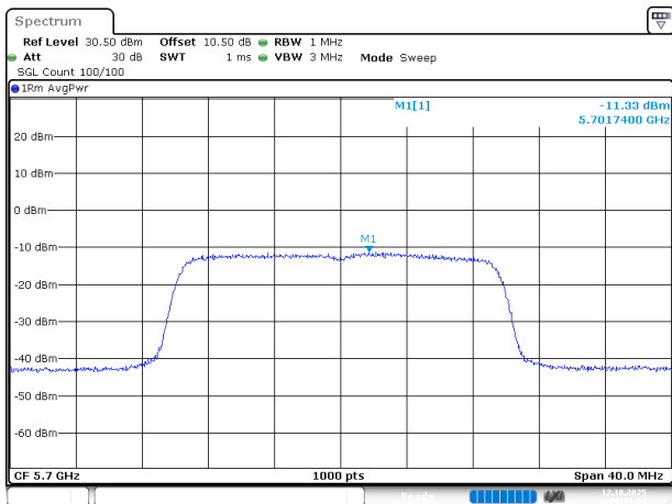
802.11ax20_5700MHz_RU_FULL_Chain 1
