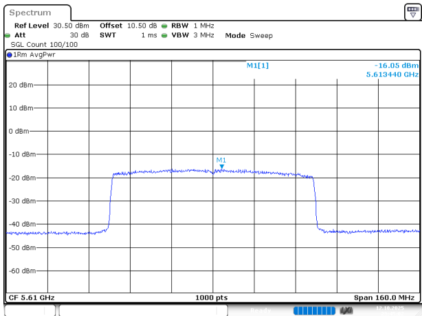
802.11ax80_5610MHz_RU_FULL_Chain 1
