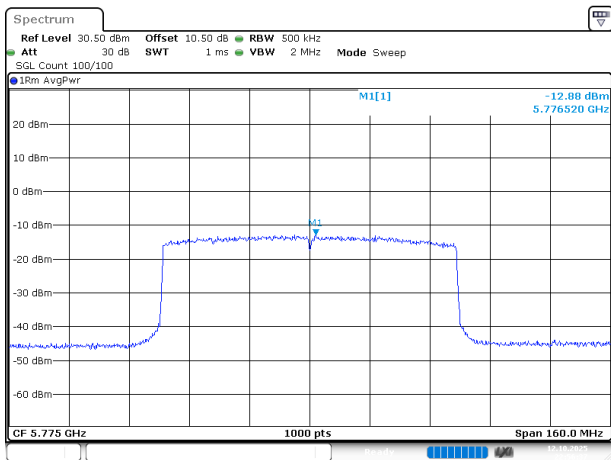
802.11ax80_5775MHz_RU_FULL_Chain 0
