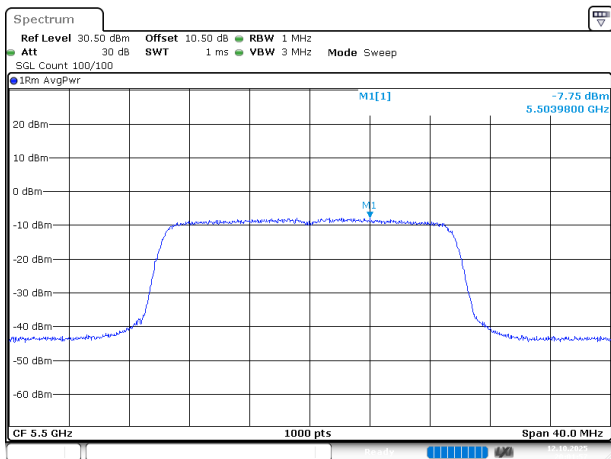
802.11ax20_5500MHz_RU_FULL_Chain 0
