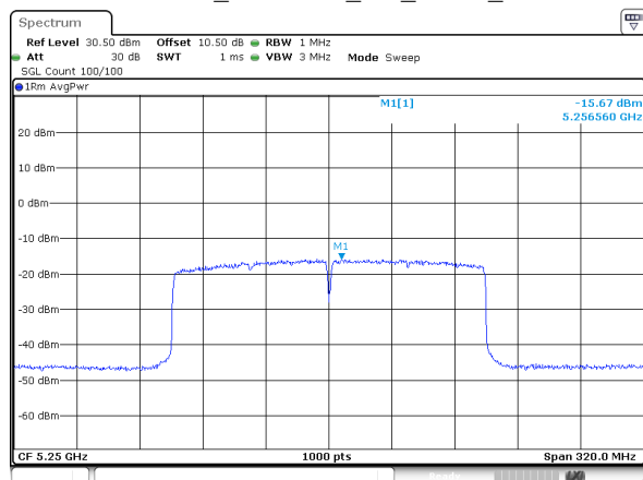
802.11ax160_5250MHz_RU_FULL_Chain 0
