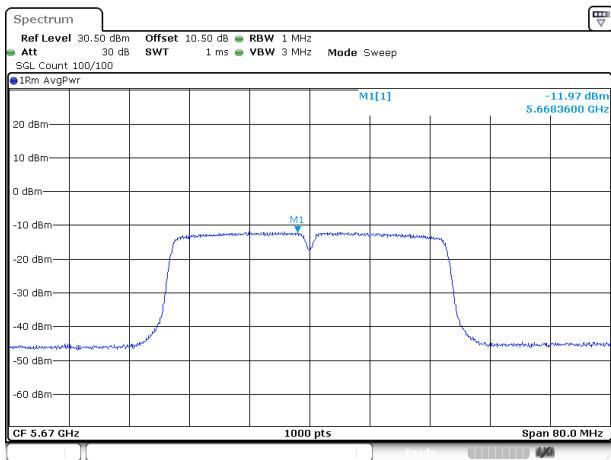
802.11ac40_5670MHz_Chain 0
