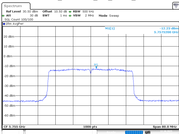
802.11ax40_5755MHz_RU_FULL_Chain 1
