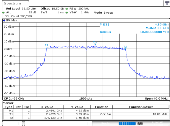
802.11ax20_2462MHz_RU_FULL_Chain 0
