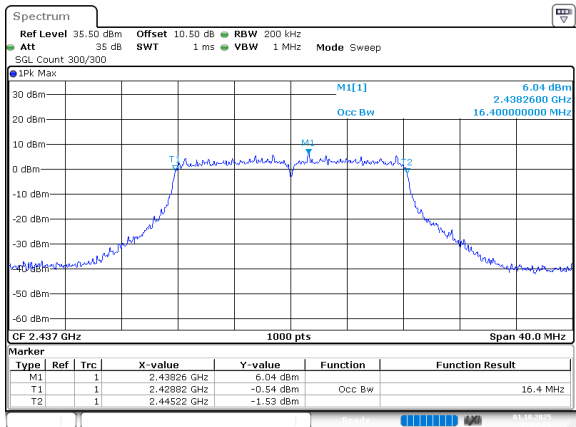
802.11g_2437MHz_Chain 0
