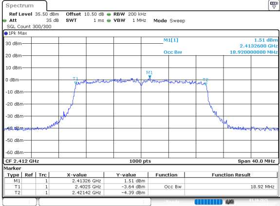
802.11ax20_2412MHz_RU_FULL_Chain 1
