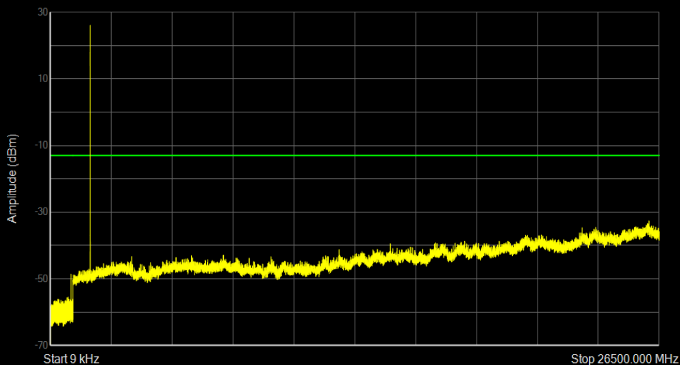
Band4 16QAM BW=1.4MHz Channel=20393 RB Size=5 Position=#0
