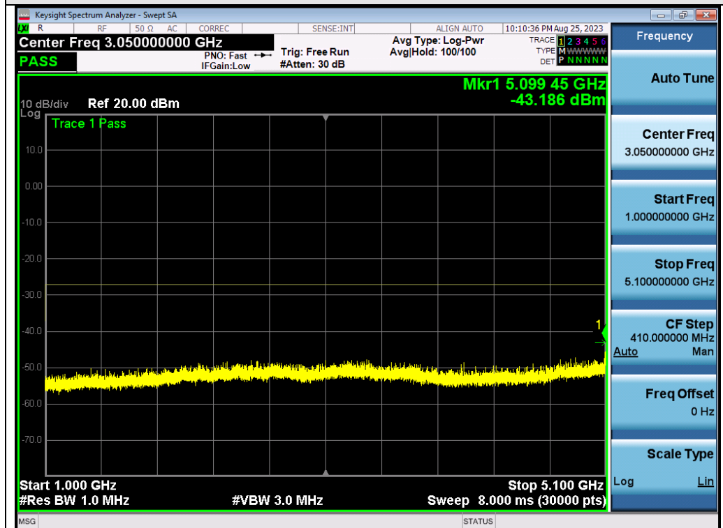
Test_Graph_802.11a_ANT2_5260_6Mbps_Frequency Band 2
