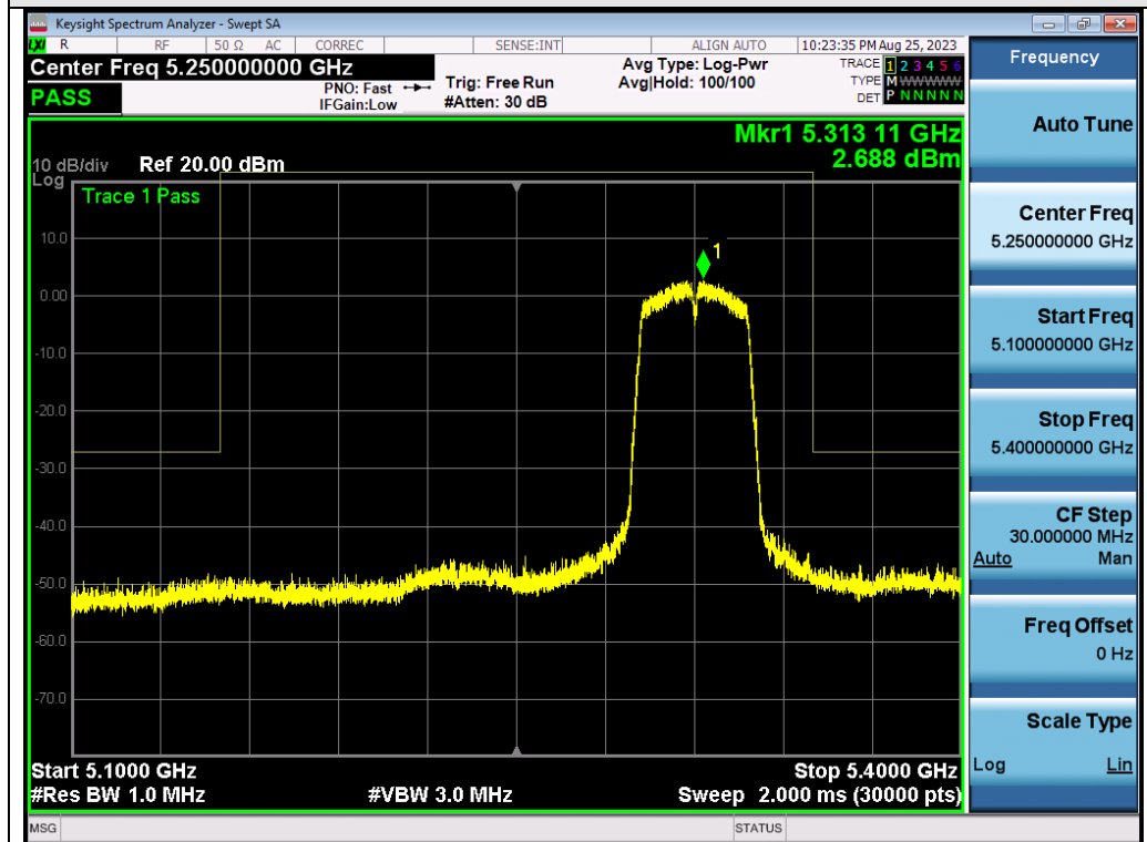
Test_Graph_802.11n40_ANT2_5310_MCS0_Frequency Band 3
