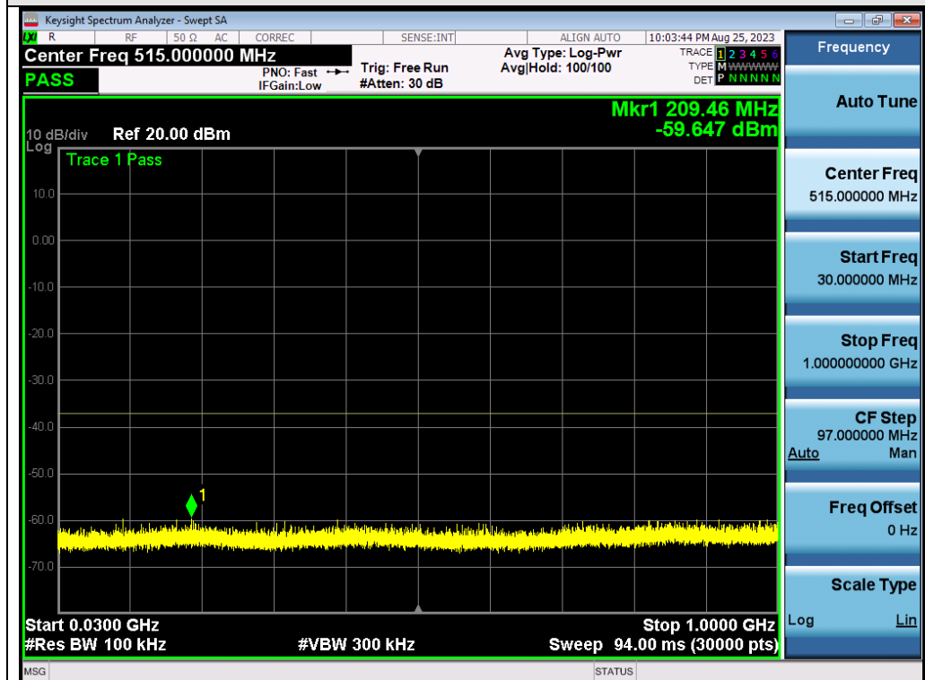
Test Graph 802.11a ANT2 5240 6Mbps Frequency Band 1
