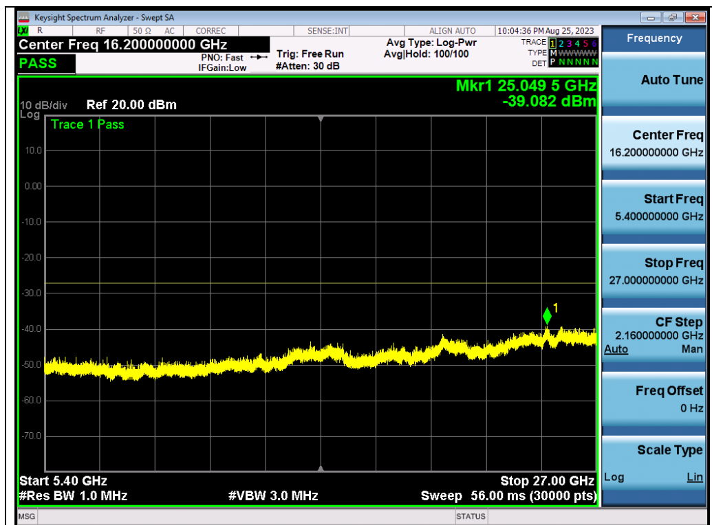
Test_Graph_802.11a_ANT2_5240_6Mbps_Frequency Band 4
