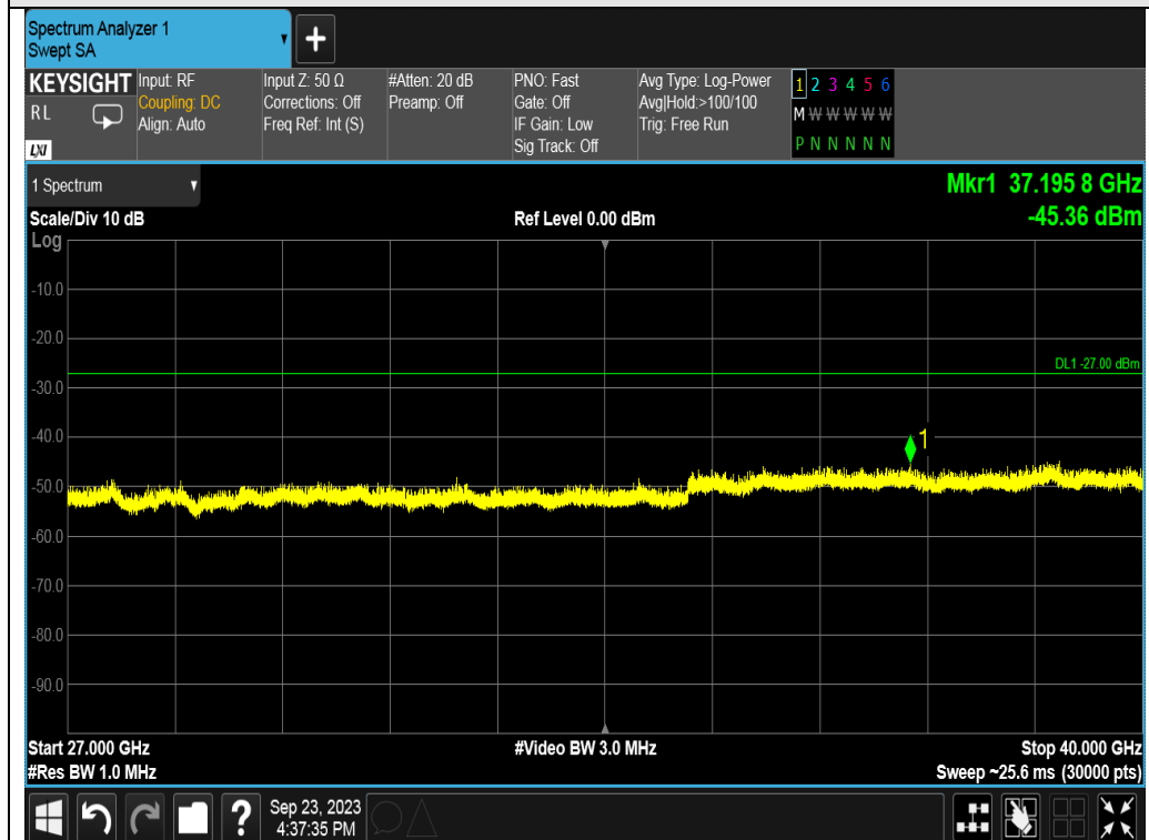
Test_Graph_802.11a_ANT2_5320_6Mbps_Frequency Band 5
