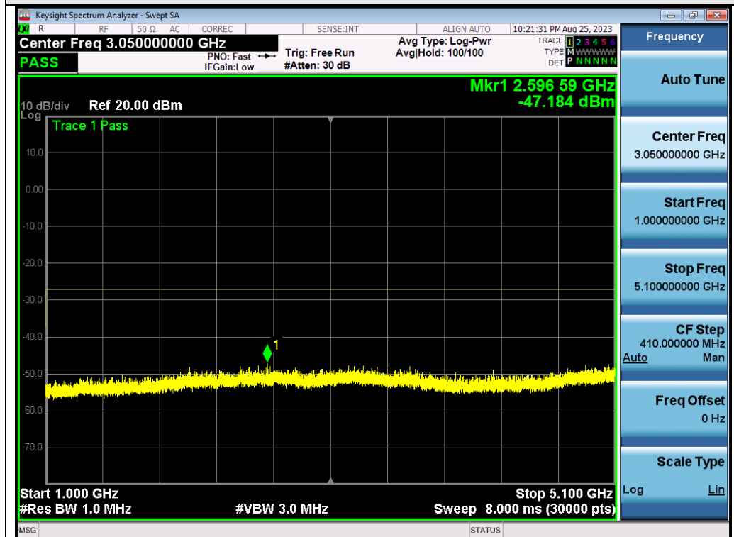
Test_Graph_802.11n40_ANT2_5270_MCS0_Frequency Band 2
