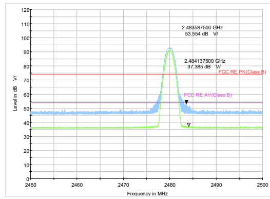
Bluetooth LE (1M) Channel 39 Peak+Average
