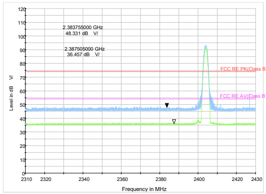
Bluetooth LE (1M) Channel 0 Peak+ Average
