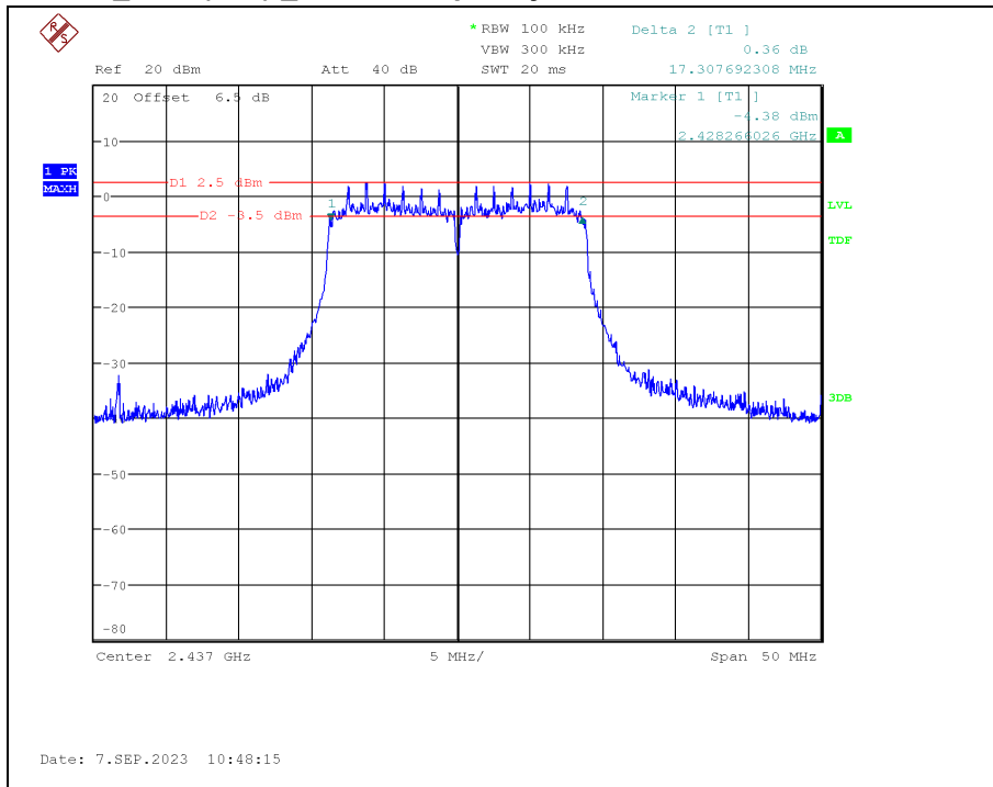
802.11n_HT20(12V) _ Middle frequency
