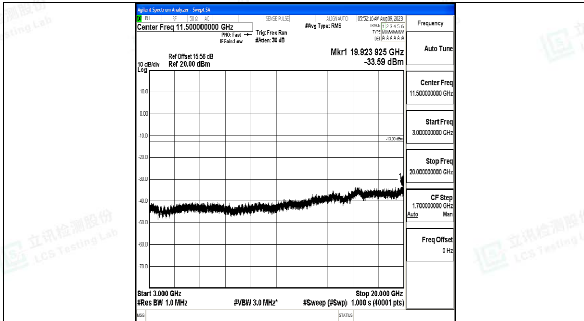
Band2_20MHz_QPSK_19100_1RB#0_3000~20000_3000~20000
