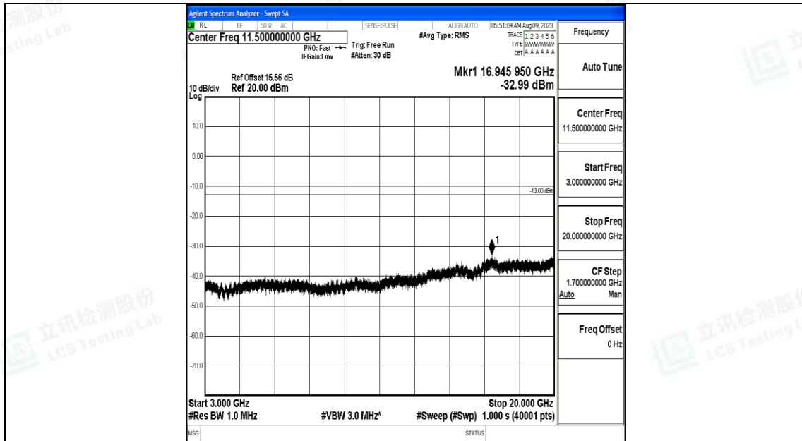
Band2_20MHz_QPSK_18900_1RB#0_3000~20000_3000~20000
