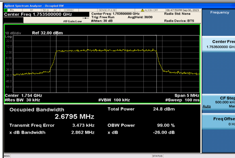
Band4-3MHz-QPSK-20385-15RB#0-2.6795
