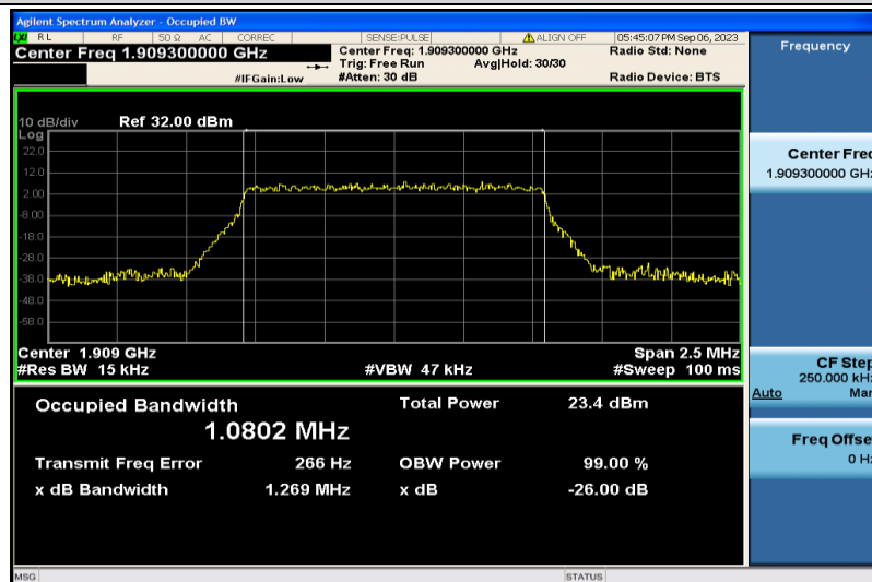
Band2-1.4MHz-16QAM-19193-6RB#0-1.0802
