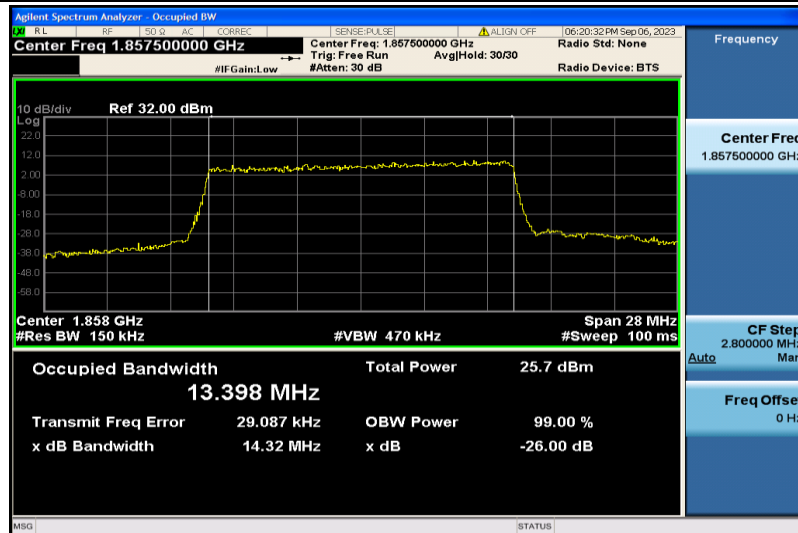
Band2-15MHz-QPSK-18675-75RB#0-13.398
