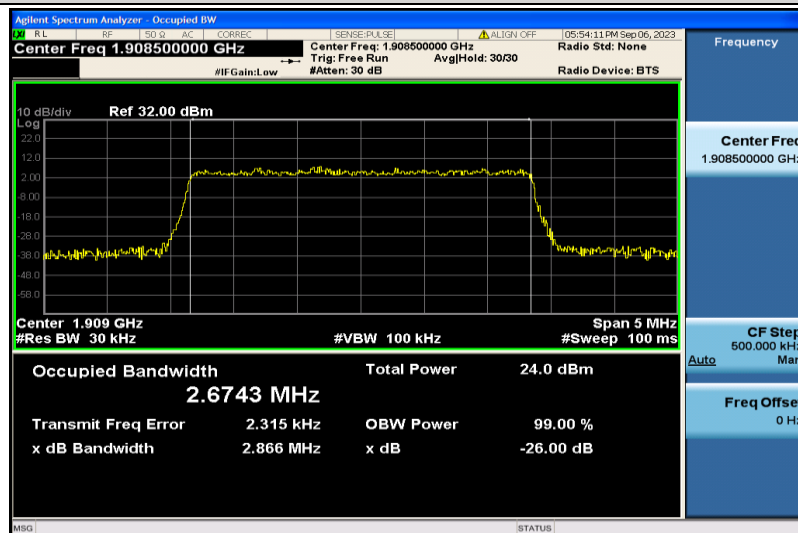
Band2-3MHz-16QAM-19185-15RB#0-2.6743
