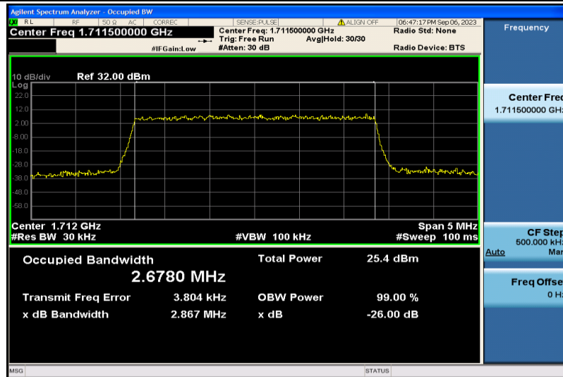
Band4-3MHz-QPSK-19965-15RB#0-2.6780
