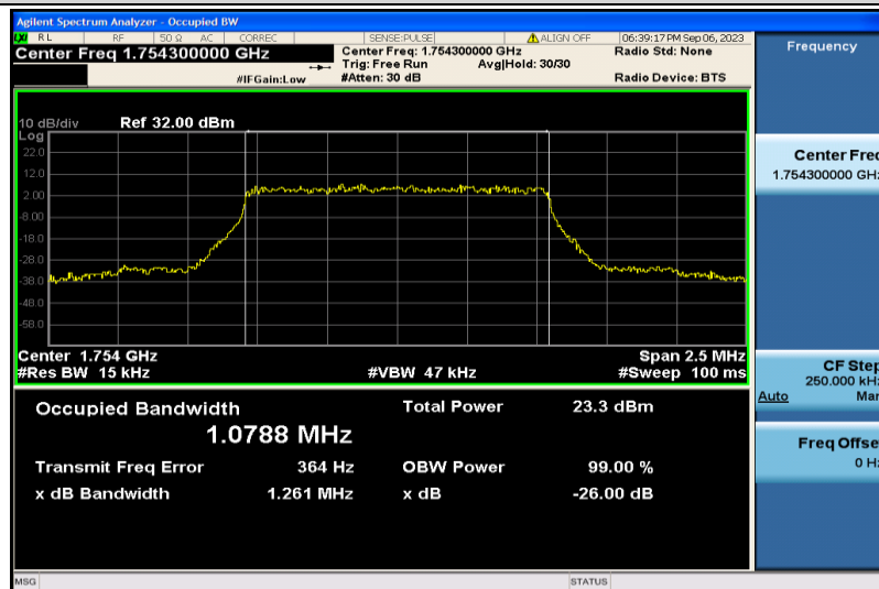
Band4-1.4MHz-16QAM-20393-6RB#0-1.0788
