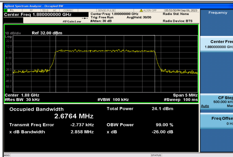
Band2-3MHz-16QAM-18900-15RB#0-2.6764
