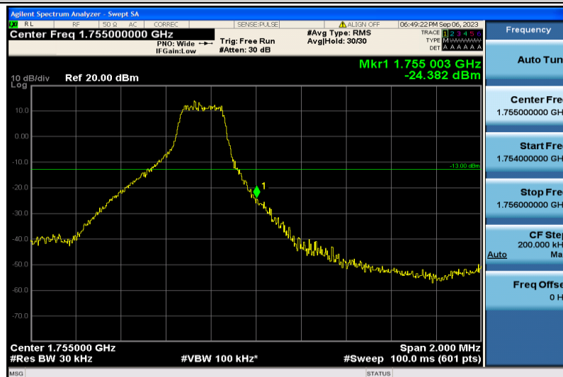
Band4-3MHz-16QAM-20385-1RB#14
