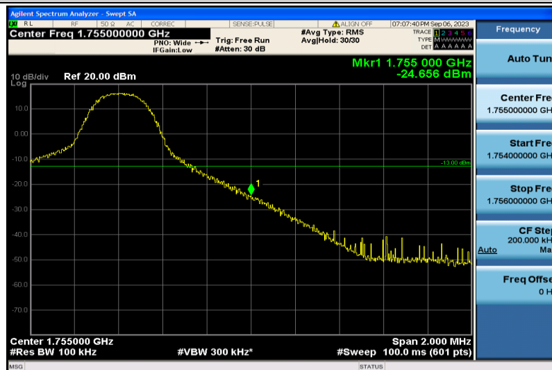
Band4-10MHz-QPSK-20350-1RB#49
