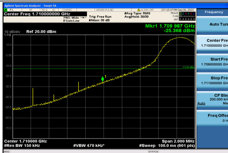
Band4-15MHz-QPSK-20025-1RB#0
