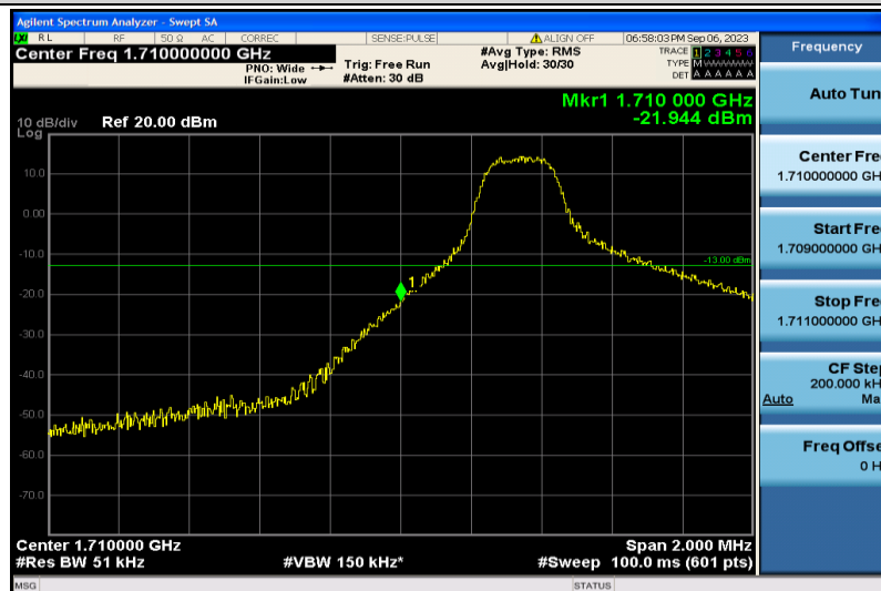
Band4-5MHz-16QAM-19975-1RB#0
