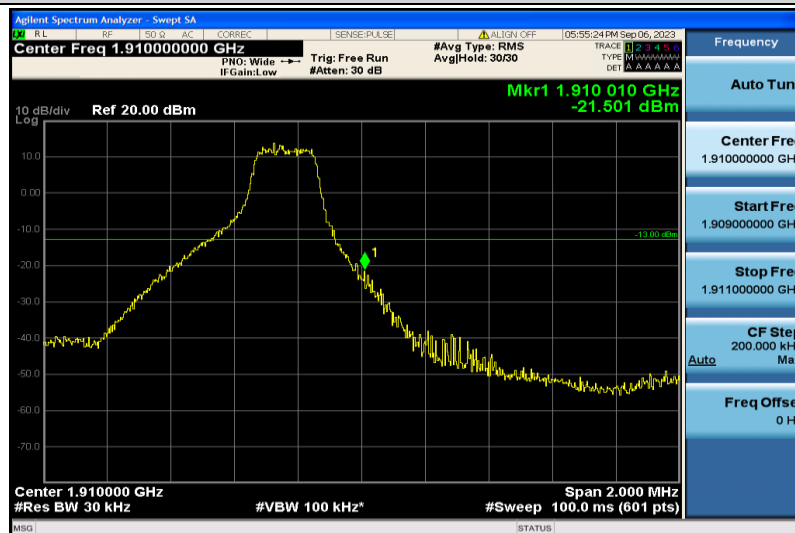
Band2-3MHz-16QAM-19185-1RB#14
