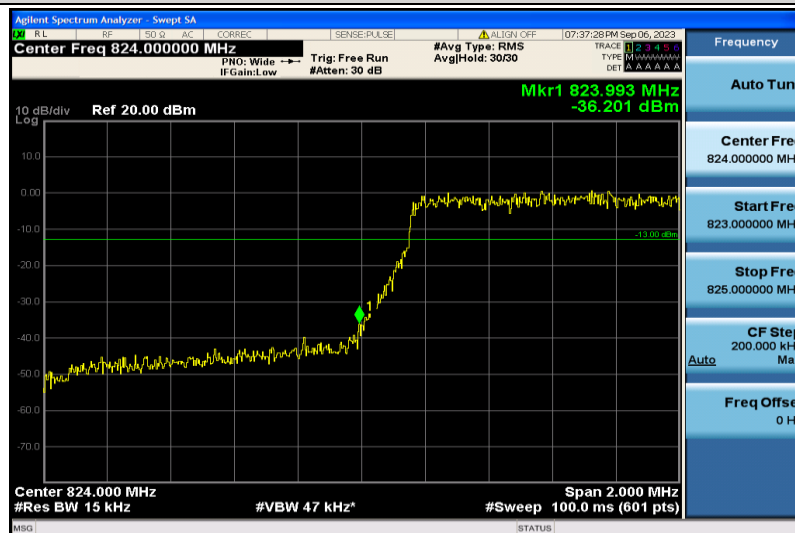
Band5-1.4MHz-16QAM-20407-6RB#0
