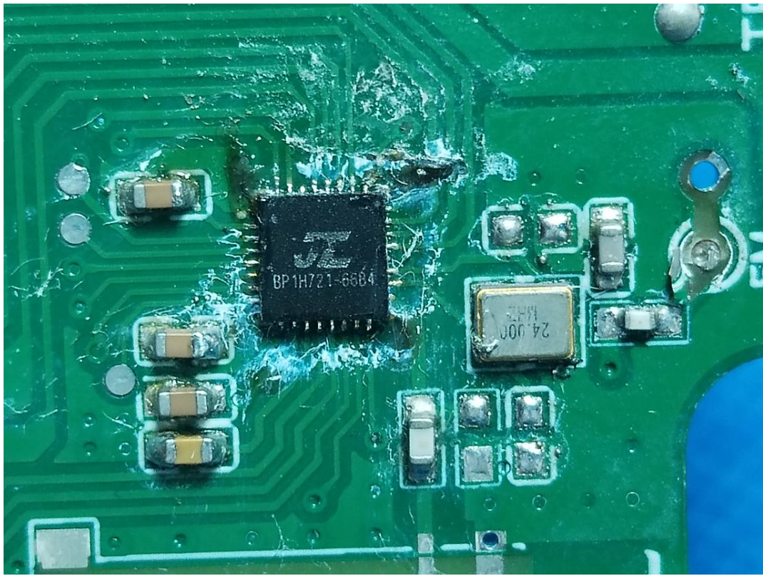
BT Antenna
