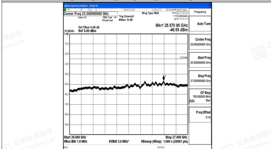
Band41_10MHz_16QAM_41190_1RB#0_20000~27000_20000~27000
