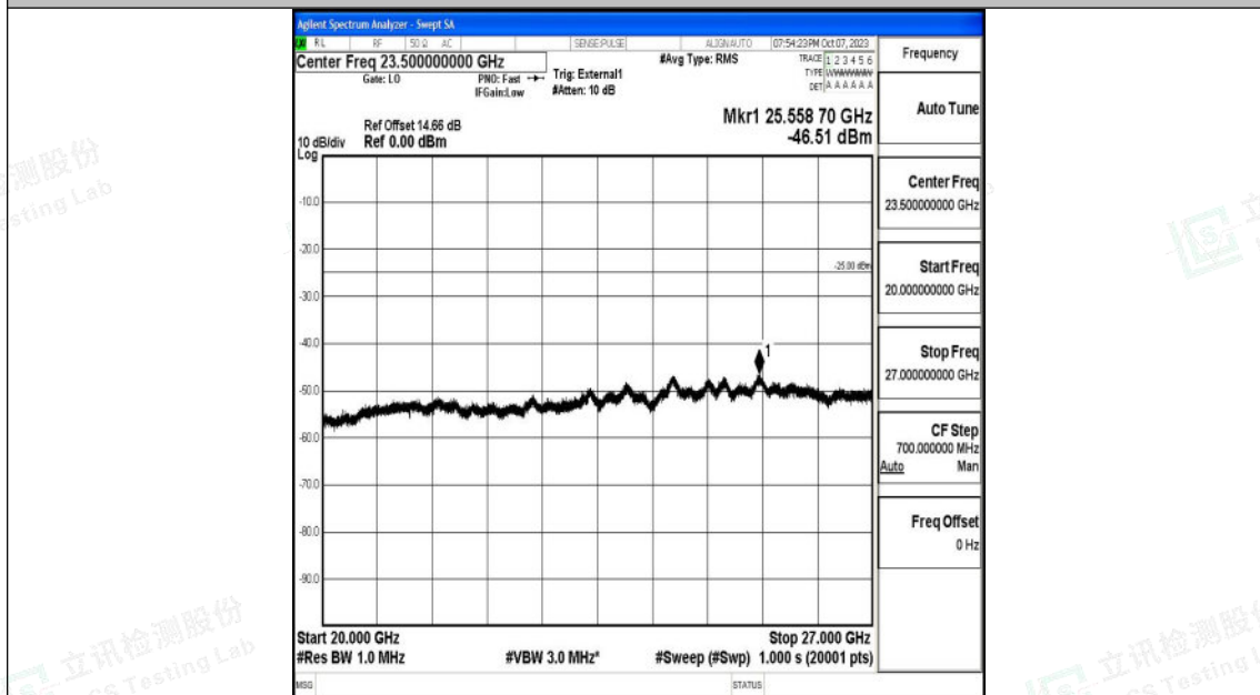
Band41_20MHz_16QAM_41140_1RB#0_20000~27000_20000~27000
