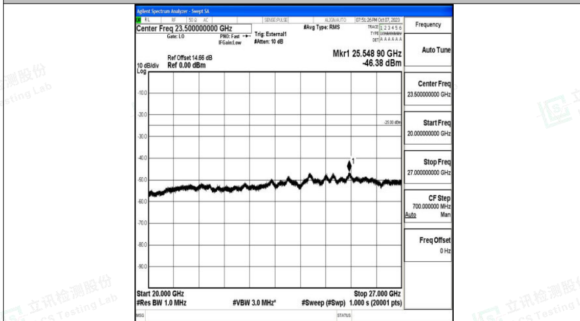
Band41_20MHz_16QAM_40590_1RB#0_20000~27000_20000~27000
