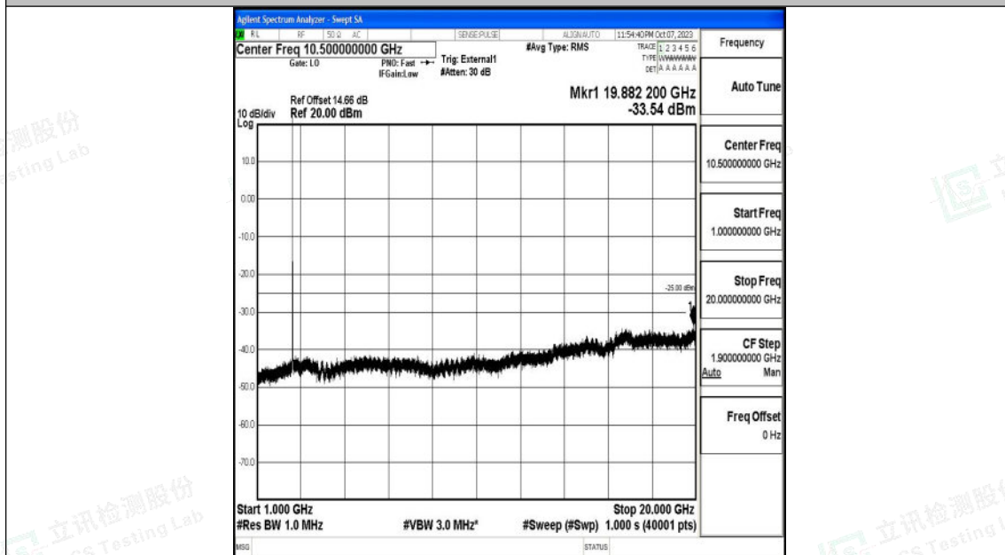
Band41_15MHz_16QAM_40115_1RB#0_1000~20000_1000~20000
