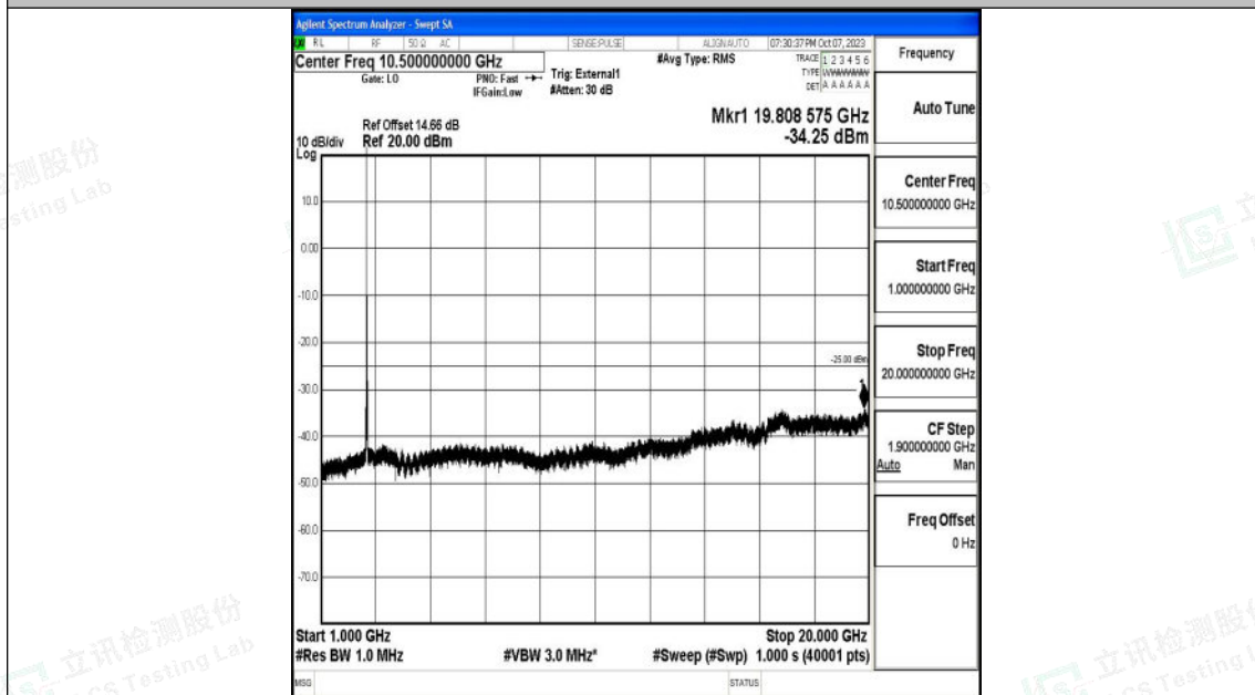
Band41_15MHz_QPSK_40590_1RB#0_1000~20000_1000~20000
