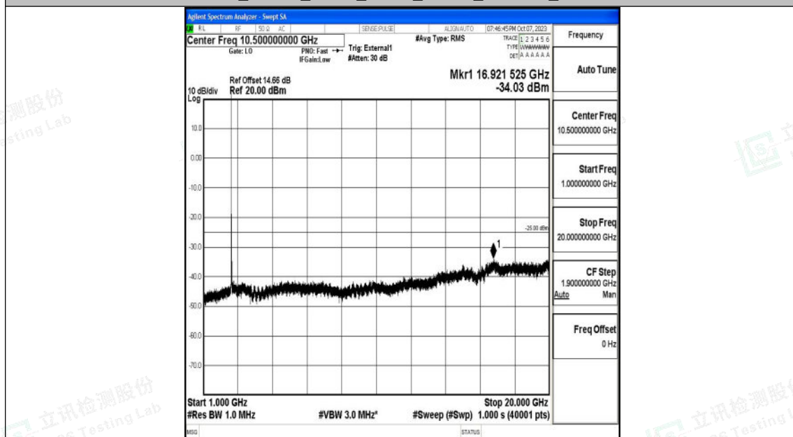
Band41_20MHz_QPSK_40140_1RB#0_1000~20000_1000~20000
