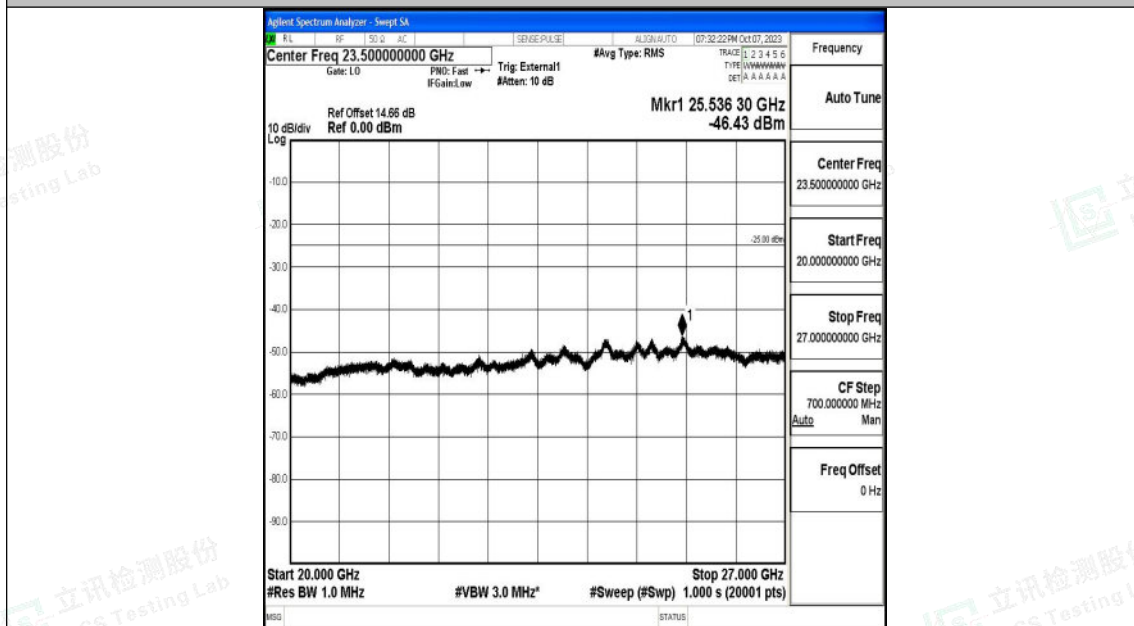
Band41_15MHz_16QAM_40590_1RB#0_20000~27000_20000~27000
