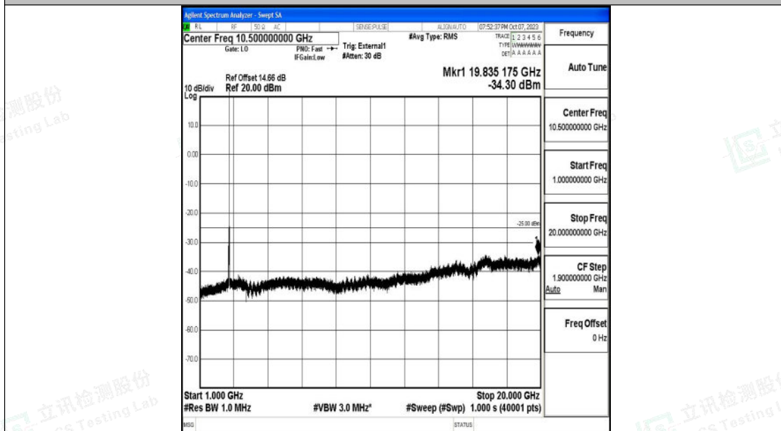
Band41_20MHz_QPSK_41140_1RB#0_1000~20000_1000~20000
