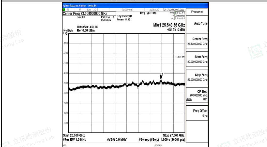
Band41_10MHz_16QAM_40590_1RB#0_20000~27000_20000~27000
