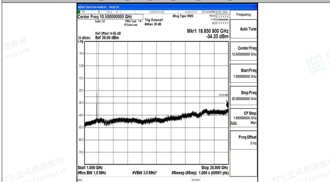
Band41_10MHz_QPSK_41190_1RB#0_1000~20000_1000~20000
