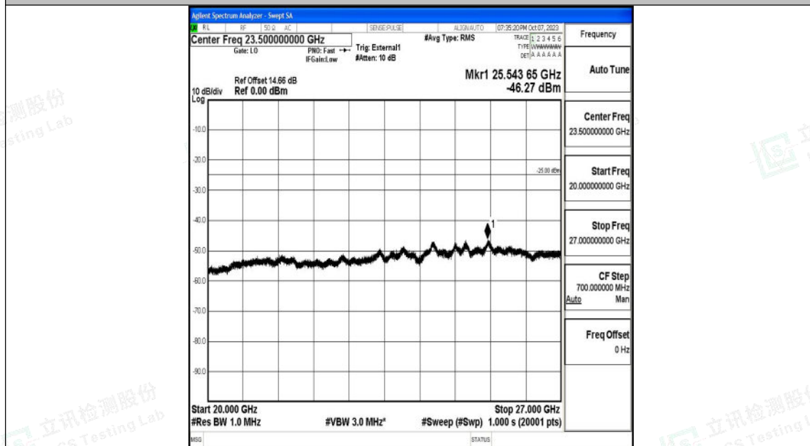
Band41_15MHz_16QAM_41165_1RB#0_20000~27000_20000~27000
