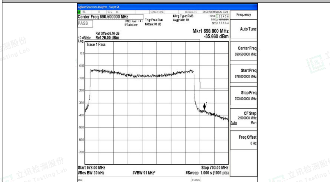
Band71_20MHz_16QAM_133372_100RB#0
