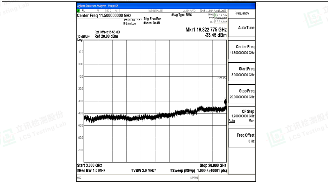
Band4_15MHz_QPSK_20325_1RB#0_3000~20000_3000~20000
