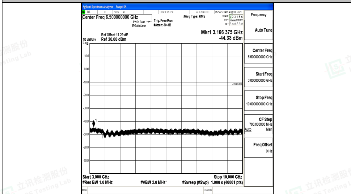
Band5_10MHz_QPSK_20450_1RB#0_3000~10000_3000~10000
