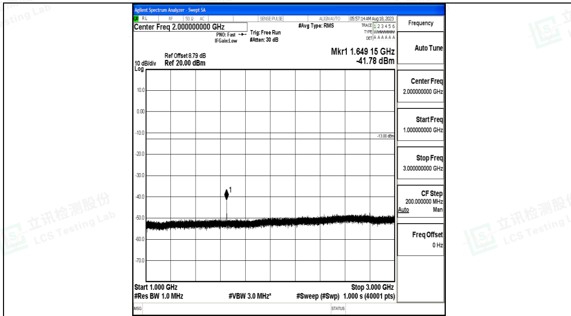
Band5_10MHz_QPSK_20450_1RB#0_1000~3000_1000~3000
