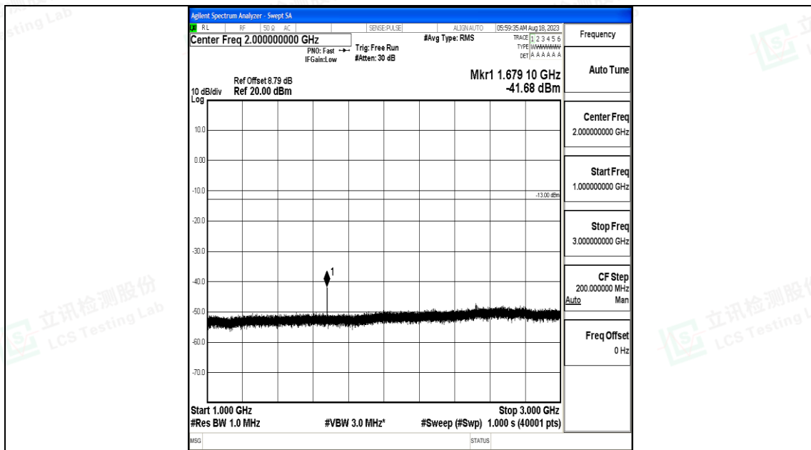
Band5_10MHz_QPSK_20600_1RB#0_1000~3000_1000~3000
