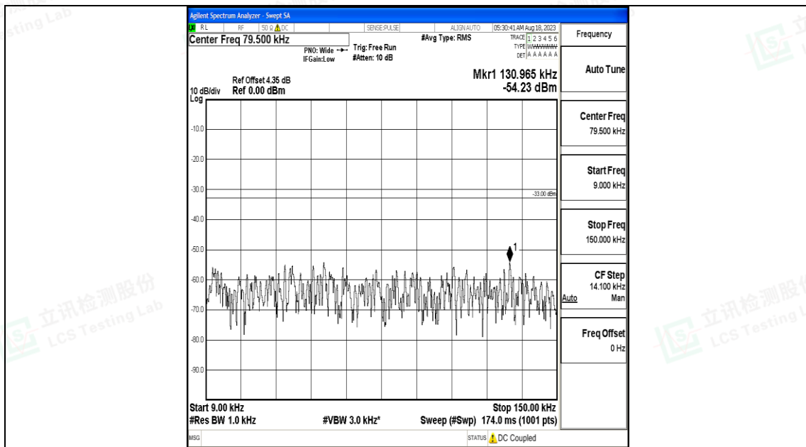
Band5_3MHz_16QAM_20525_1RB#0_0.009~0.15_0.009~0.15
