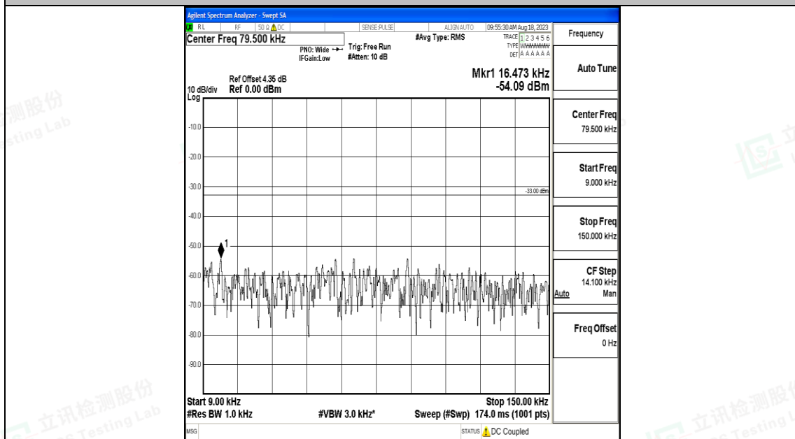
Band26_10MHz_16QAM_26740_1RB#0_0.009~0.15_0.009~0.15
