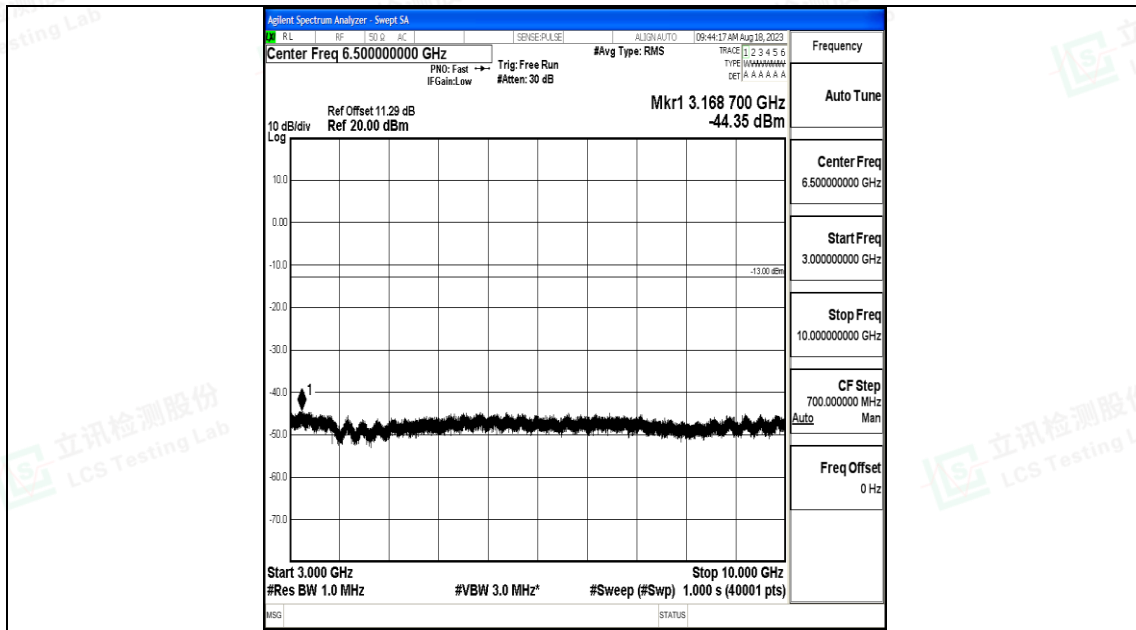
Band26_5MHz_QPSK_26715_1RB#0_3000~10000_3000~10000
