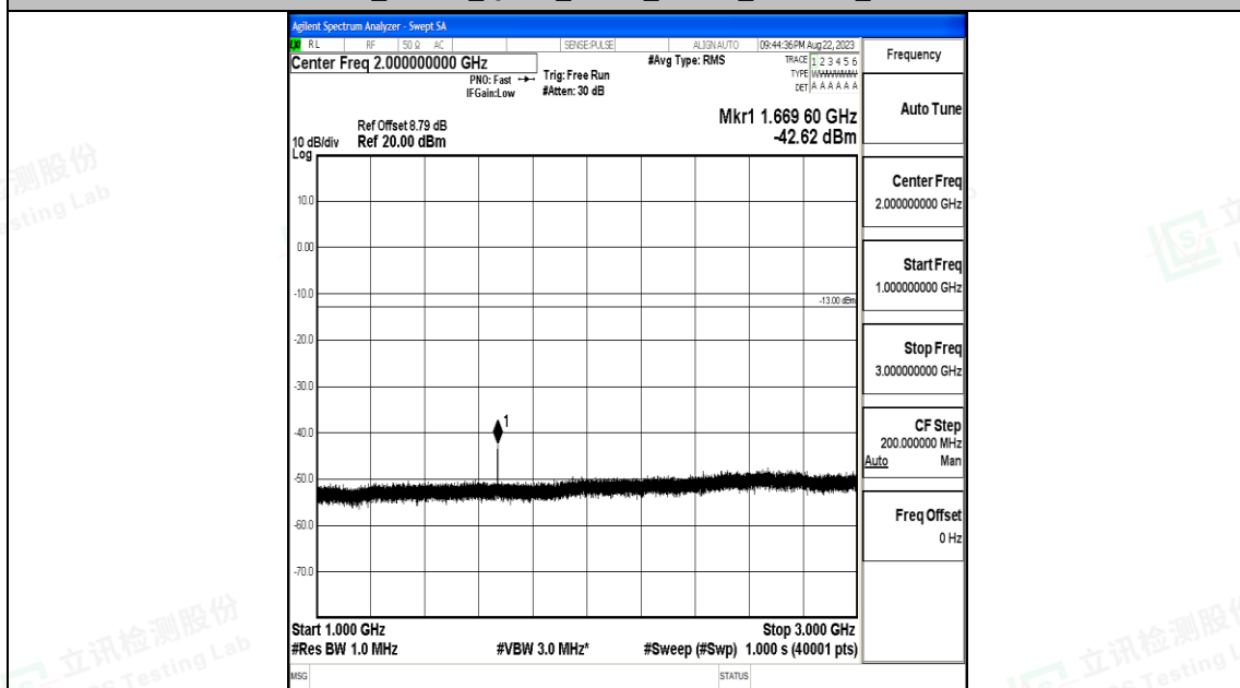
Band26_15MHz_QPSK_26965_1RB#0_1000~3000_1000~3000
