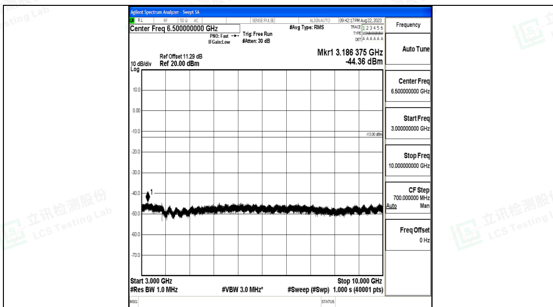
Band26_15MHz_QPSK_26865_1RB#0_3000~10000_3000~10000
