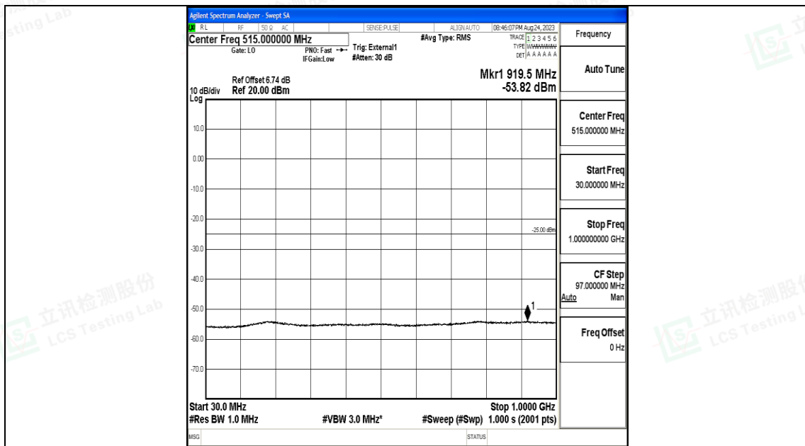
Band41_15MHz_QPSK_40620_1RB#0_30~1000_30~1000
