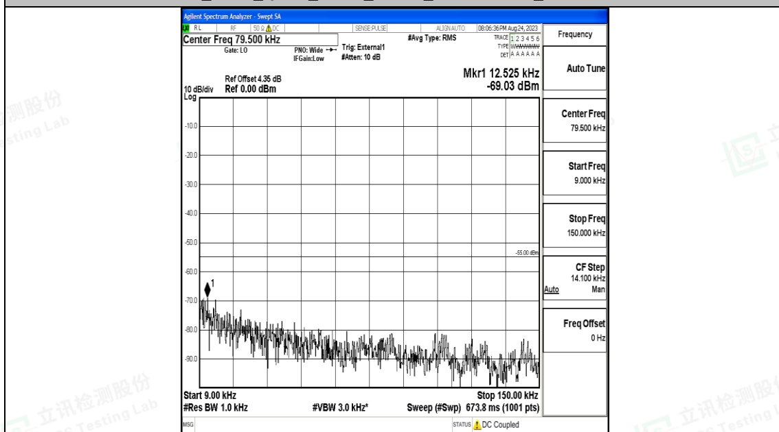
Band41_5MHz_16QAM_41565_1RB#0_0.009~0.15_0.009~0.15
