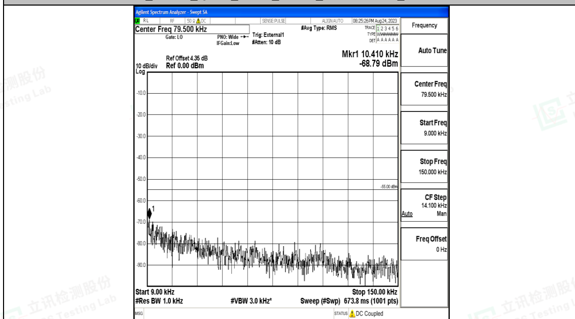
Band41_10MHz_16QAM_41540_1RB#0_0.009~0.15_0.009~0.15
