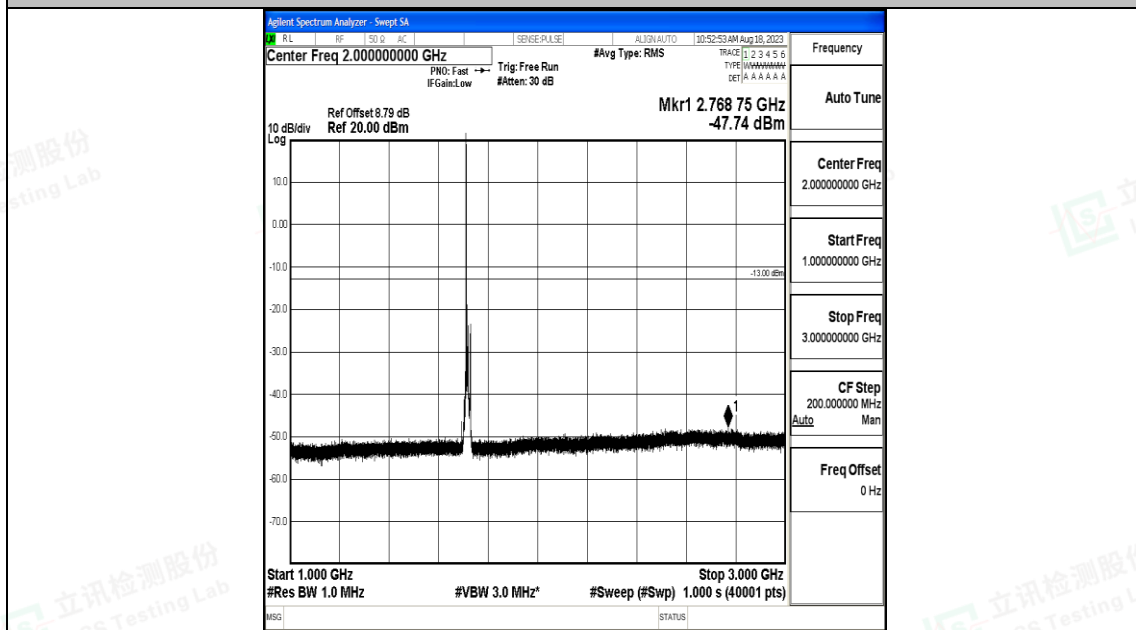
Band66_10MHz_QPSK_132022_1RB#0_1000~3000_1000~3000
