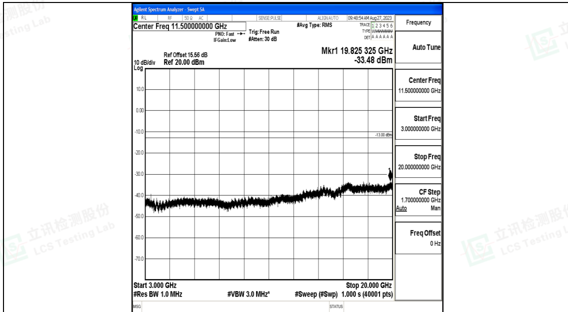
Band4_10MHz_QPSK_20000_1RB#0_3000~20000_3000~20000
